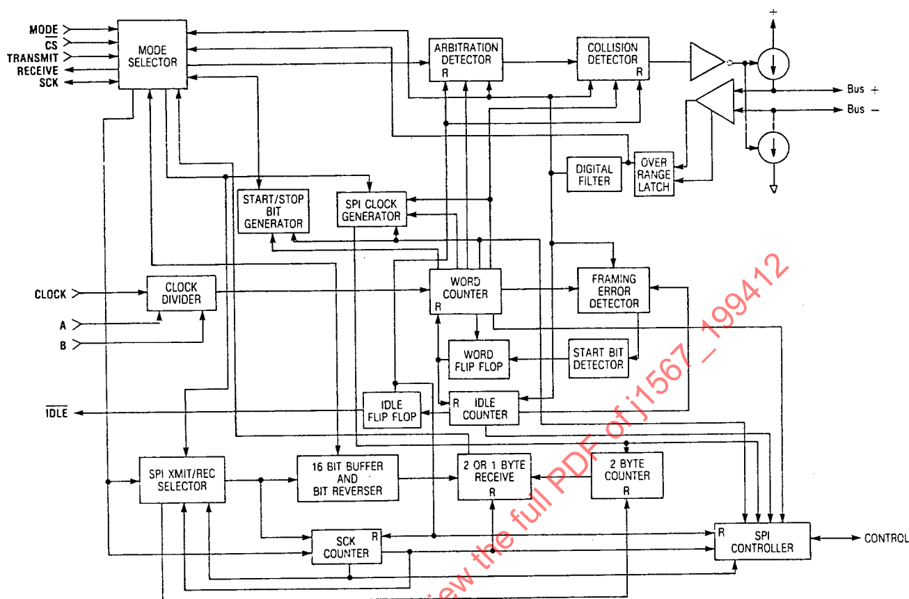
FIG. 3 - BLOCK DIAGRAM OF UNIVERSAL BUS INTERFACE IC
