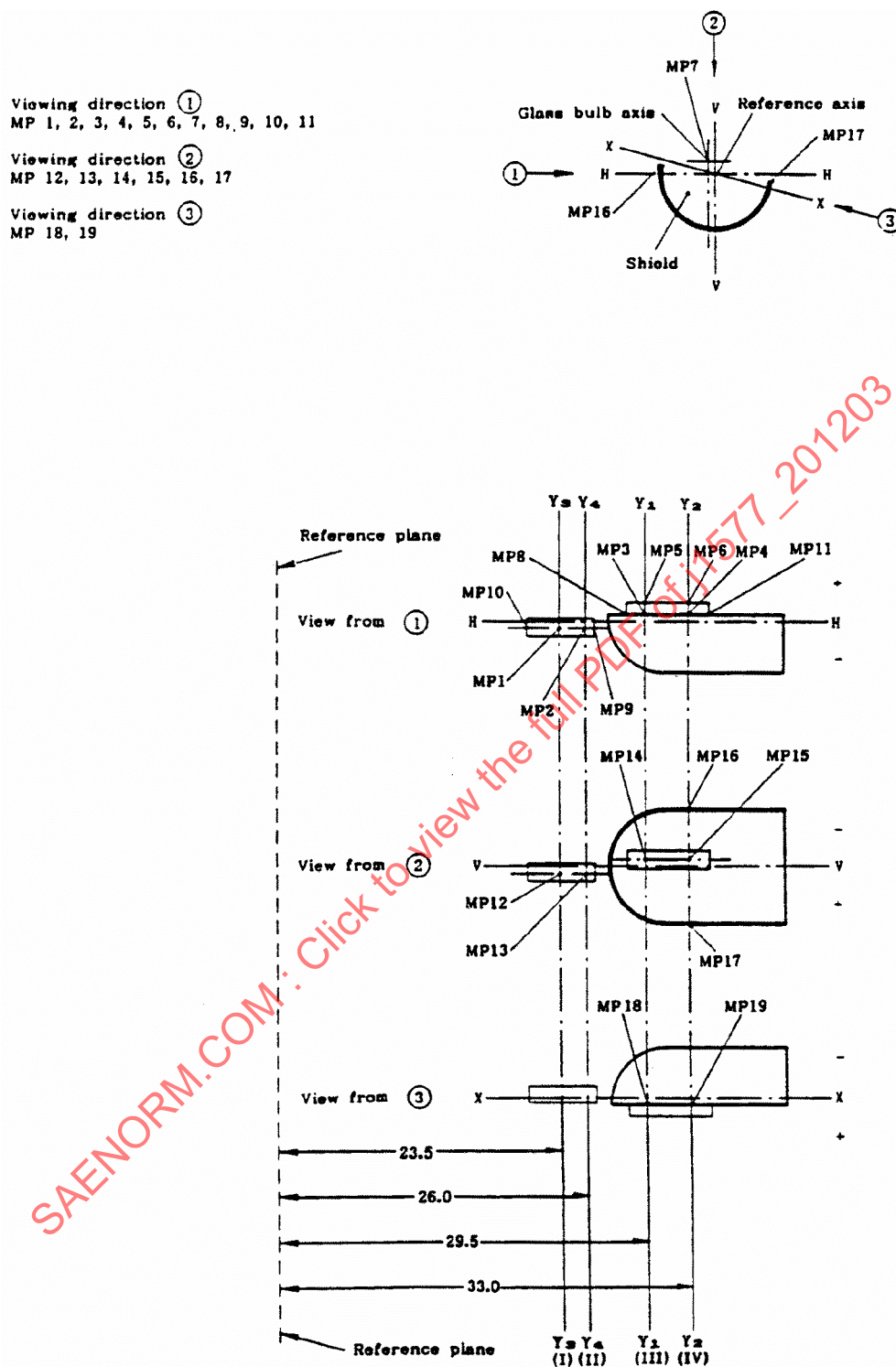
FIGURE 8—SPECIFICATION FOR THE TYPE H4/HB2 REPLACEABLE BULB— POSITIONS OF MEASURING POINTS OF H4/HB2 BULBS
