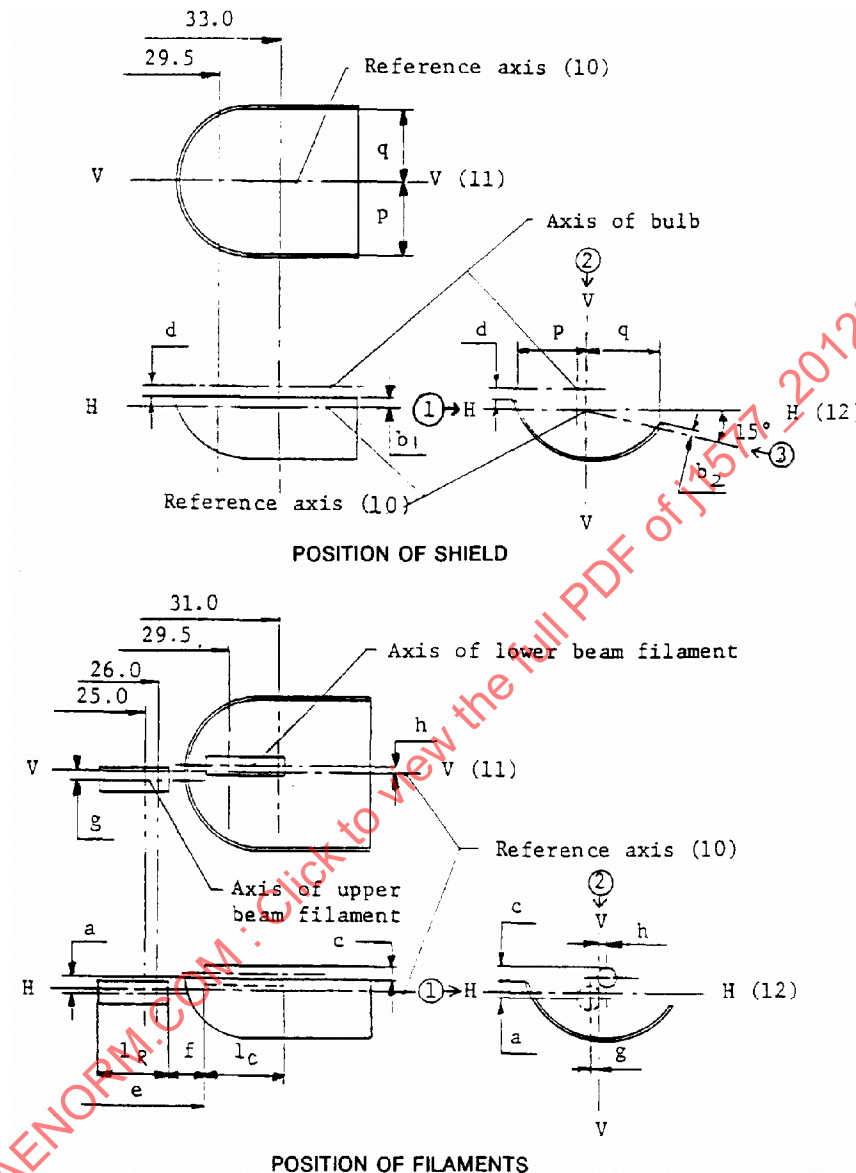
FIGURE 10—TYPE HS1 REPLACEABLE MOTORCYCLE HEADLAMP BULB— SHIELD AND FILAMENT POSITION DIMENSIONAL SPECIFICATIONS
