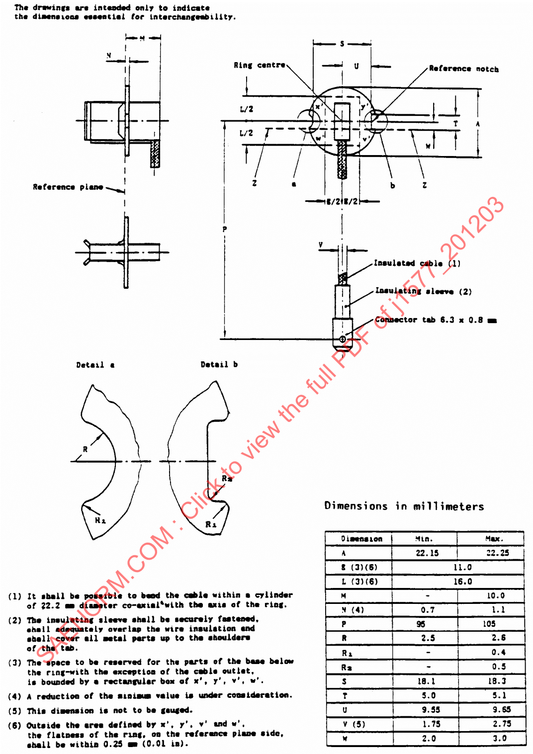
FIGURE 18—SPECIFICATION FOR THE TYPE H3 REPLACEABLE BULB BASE PK22S
