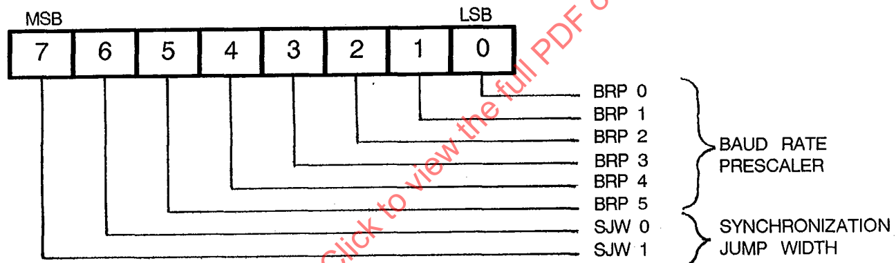
FIGURE A6 - Bus Timing Register 0 (03H)
