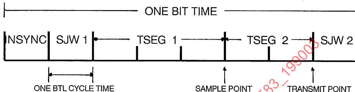
FIGURE 12 - Bit Segments
