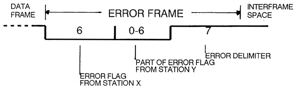
FIGURE 9 - Error Frame
