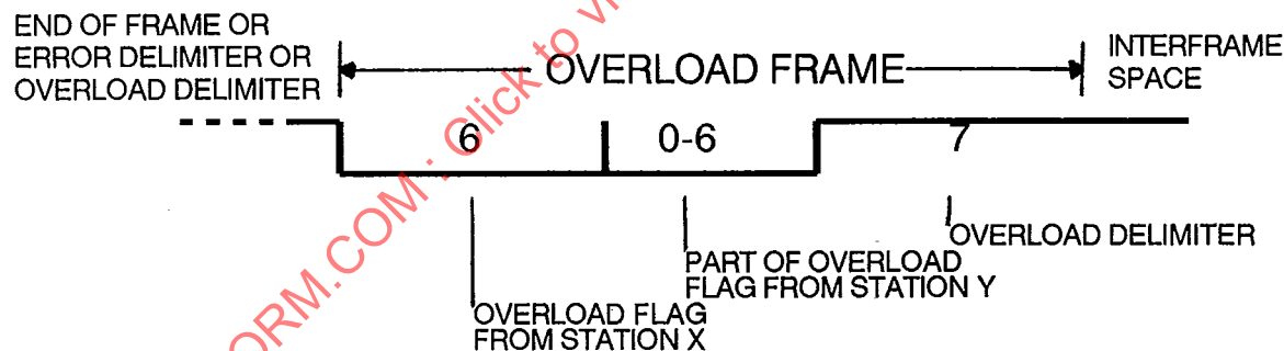
FIGURE 10 - Overload Frame
