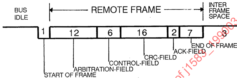
FIGURE 8 - Remote Frame
