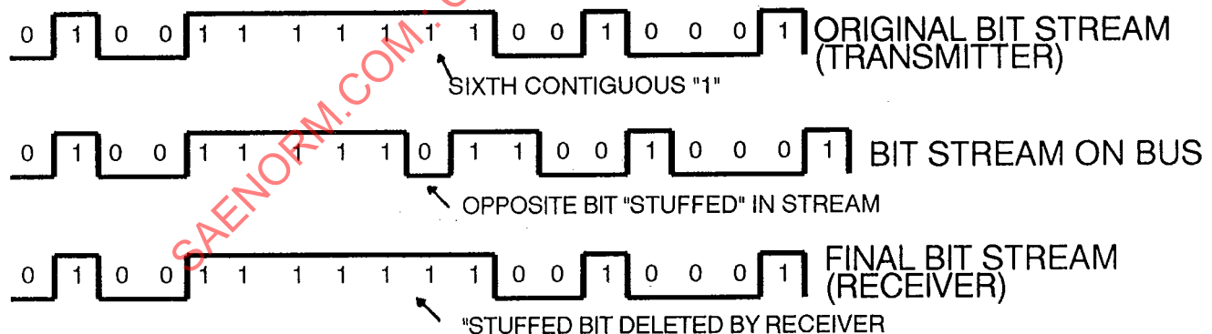
FIGURE 1 - Bit Stuffing
