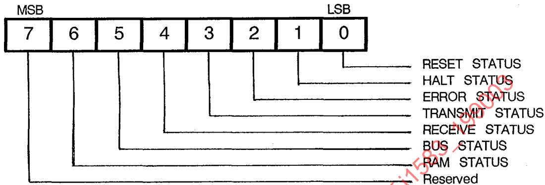
FIGURE A4 - Status Register
