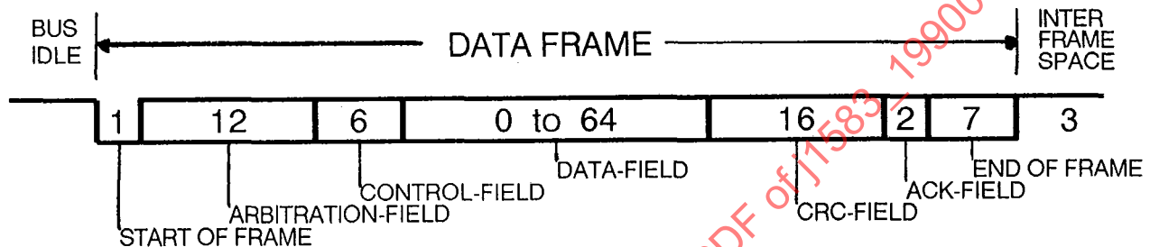
FIGURE 2 - Data Frame
