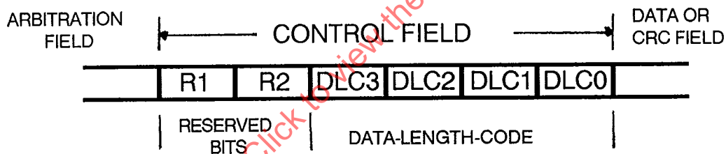
FIGURE 4 - Control Field
