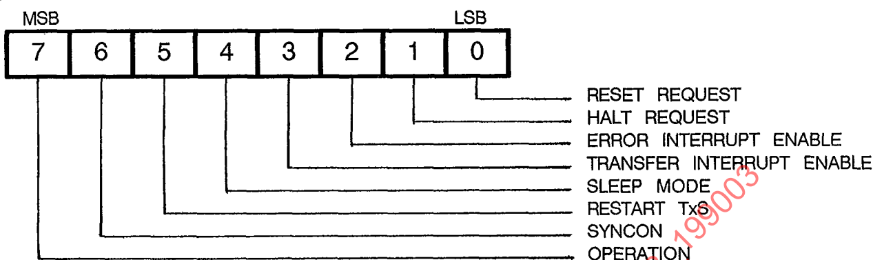
FIGURE A3 - Control Register (00h)
