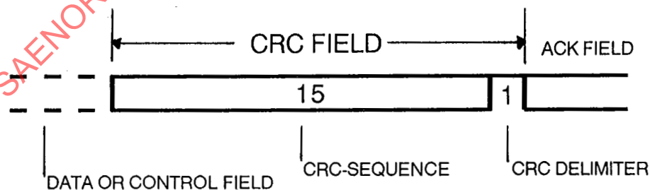
FIGURE 6 - CRC Field
