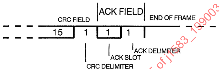
FIGURE 7 - Acknowledgement Field
