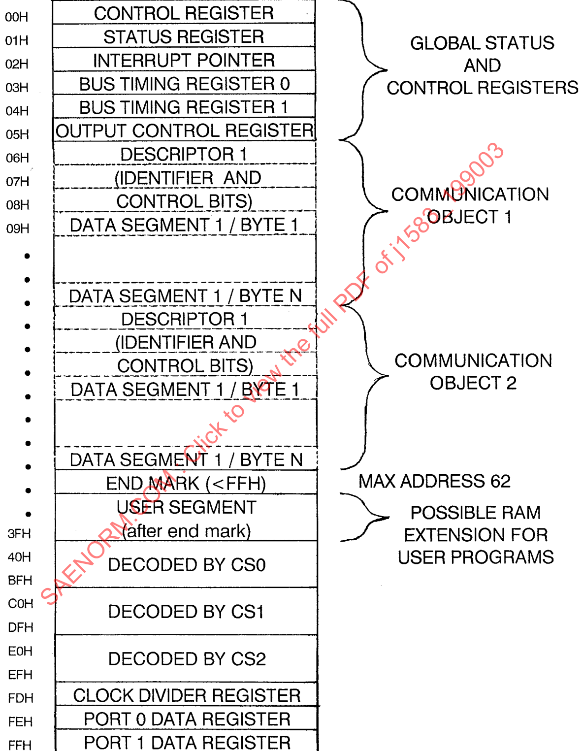
FIGURE A2 - Buffer Memory Layout
