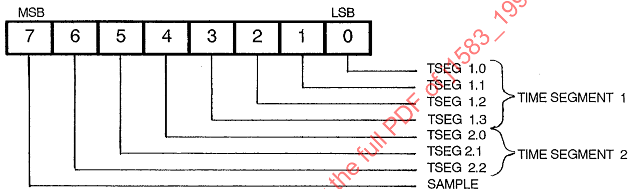
FIGURE A8 - Bus Timing Register 1 (04H)
