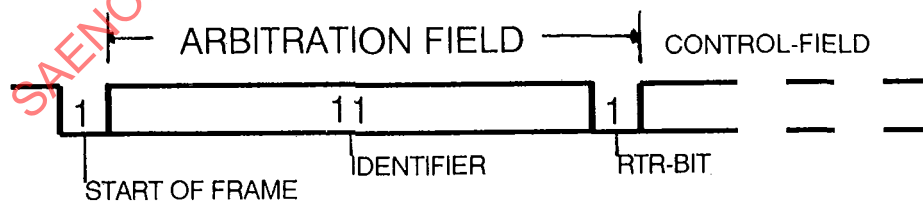
FIGURE 3 - Arbitration Field
