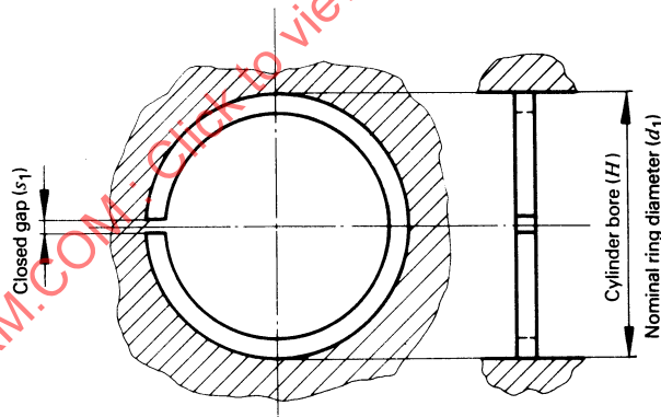
FIGURE 4—CLOSED RING
