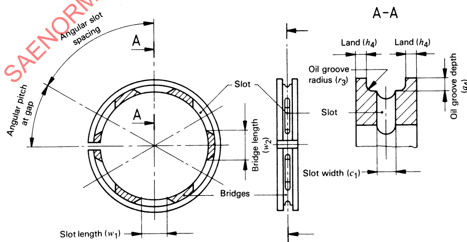
FIGURE 9—SLOTTED OIL CONTROL RING
