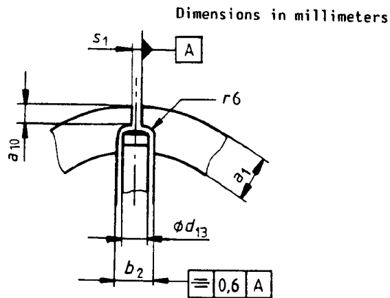
FIGURE 2—INTERNAL NOTCH—OPTION FOR PISTON RINGS WITH RADIAL WALL THICKNESS a_1 > 2.1
