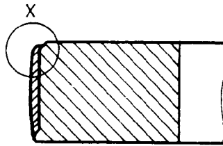
FIGURE 5—CHROMIUM COATED RING OF SEMI-INLAID DESIGN, CODE CR1E TO CR4E
