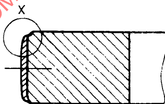
FIGURE 4—CHROMIUM COATED RING OF FULLY FACED DESIGN, CODE CRF TO CR4
