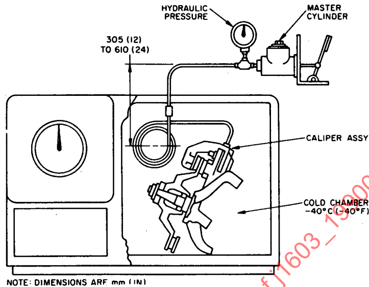
FIGURE 2 - Low Temperature Leakage Test
