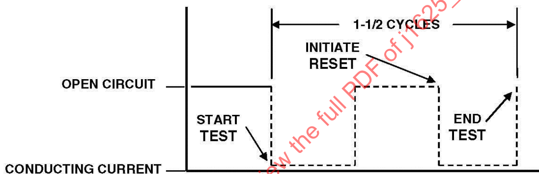
FIGURE 4—INTERRUPT CYCLE DEFINITION
