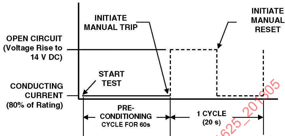
FIGURE 3—CYCLING ENDURANCE TEST CYCLE PROFILE
