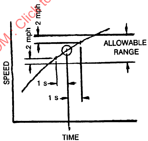
FIGURE 1—ALLOWABLE SPEED RANGE ON DRIVING SCHEDULES
