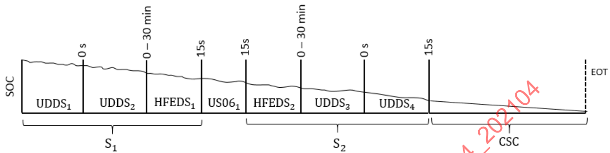
Figure 11 - SMCT+ test sequence
