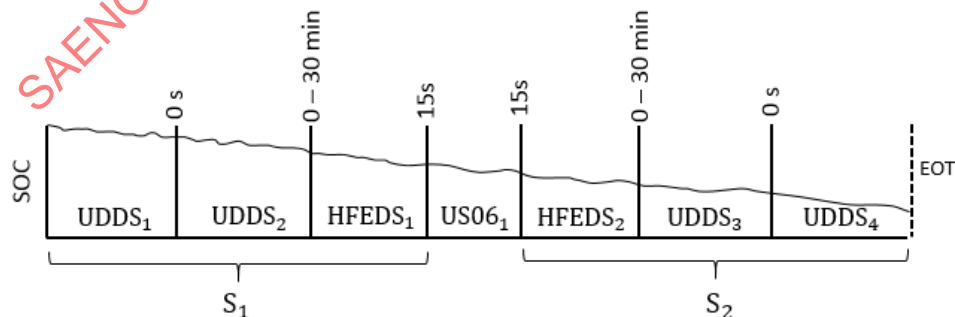
Figure 8 - SMCT test sequence
