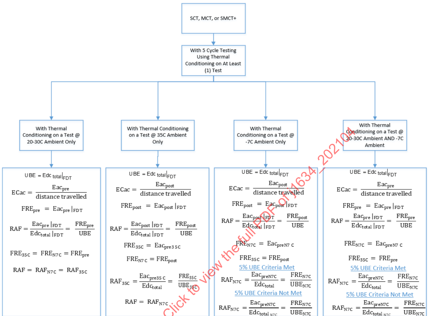
Figure B1 - Examples - equation criteria flow chart: SCT, MCT, SMCT+ utilizing thermal conditioning
