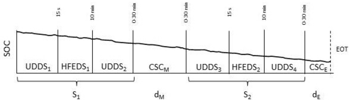
Figure 5 - Multi-cycle range test sequence
