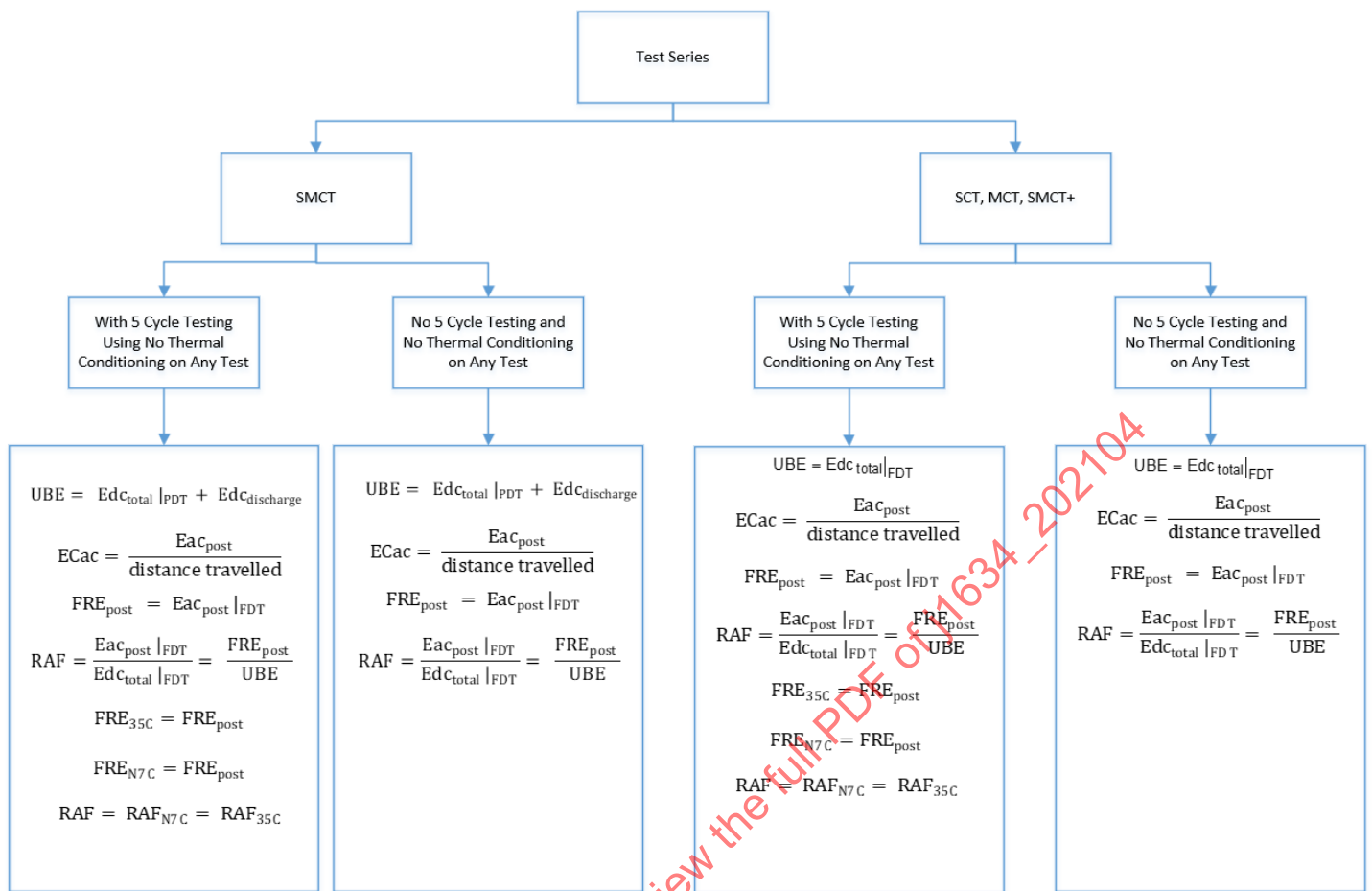
Figure B3 - Examples - equation criteria flow chart: not utilizing thermal conditioning
