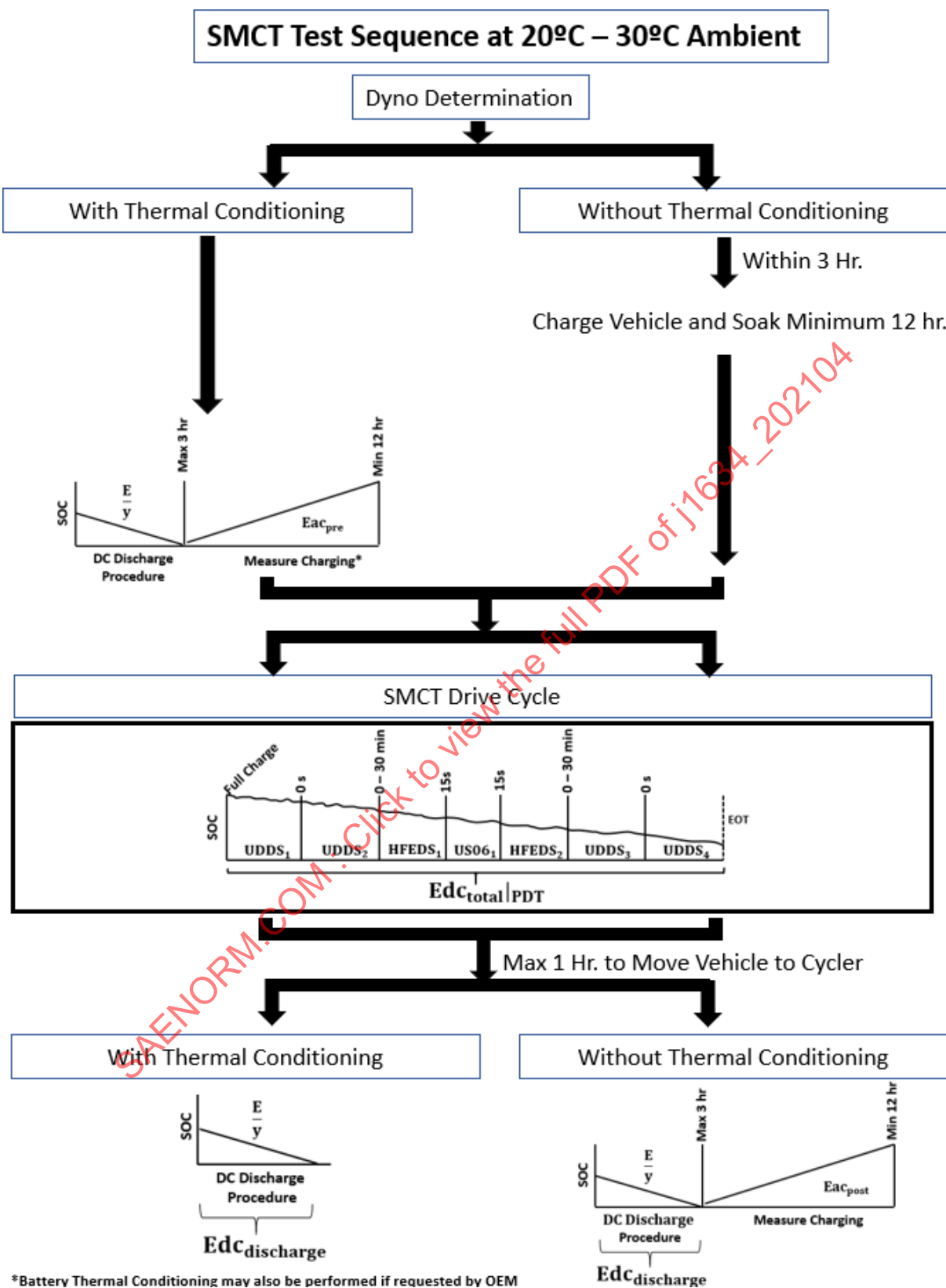
Figure 9 - Complete SMCT test sequence
