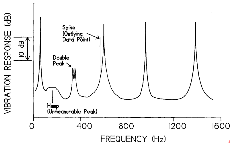
Figure 5 - Possible frequency response of a damped bar
