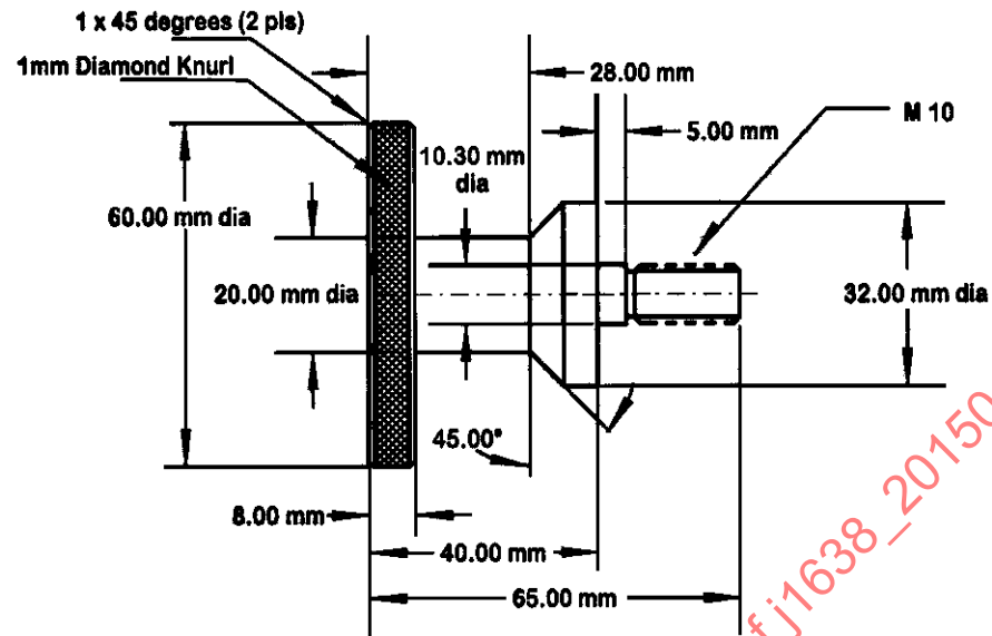
Loading Screw
