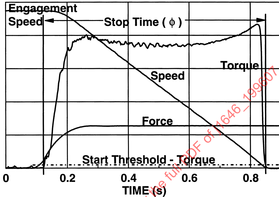
FIGURE 2—DYNAMIC ENGAGEMENT
