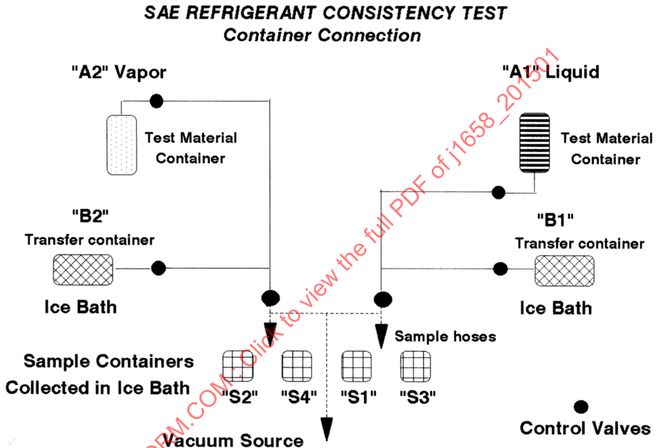
FIGURE 1—SAE REFRIGERANT CONSISTENCY TEST
