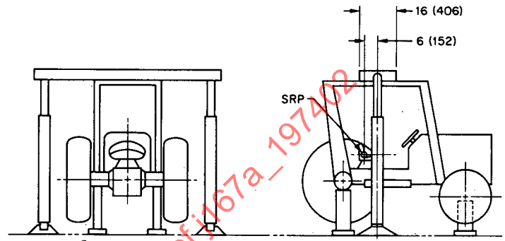
FIG. 3—METHOD OF LOAD APPLICATION FOR CRUSH TEST
