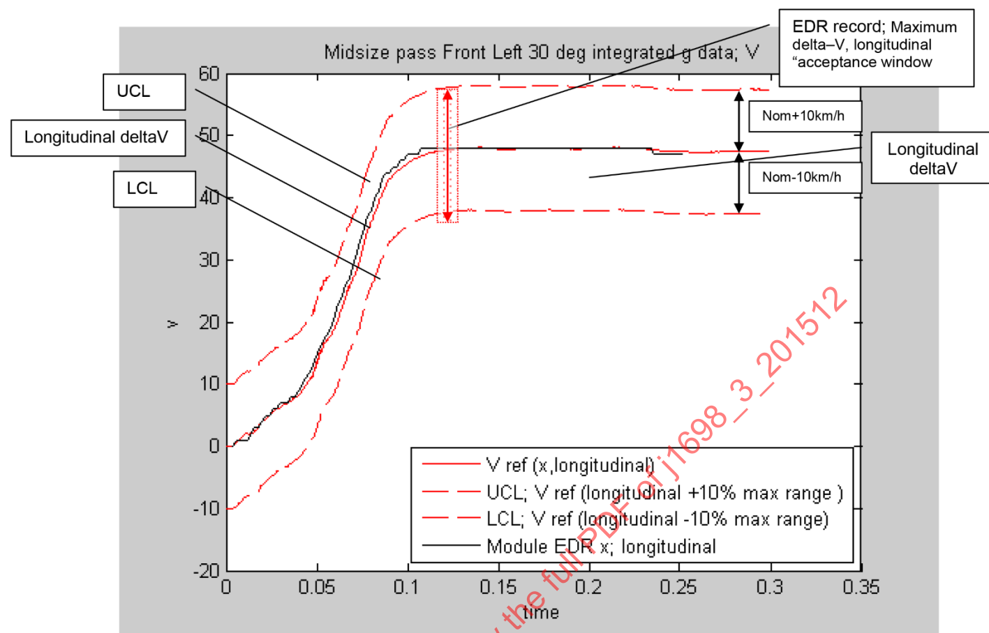
Figure 8 - Example (x) delta velocity signal with UCL and LCL and EDR data; with Maximum Delta V longitudinal
