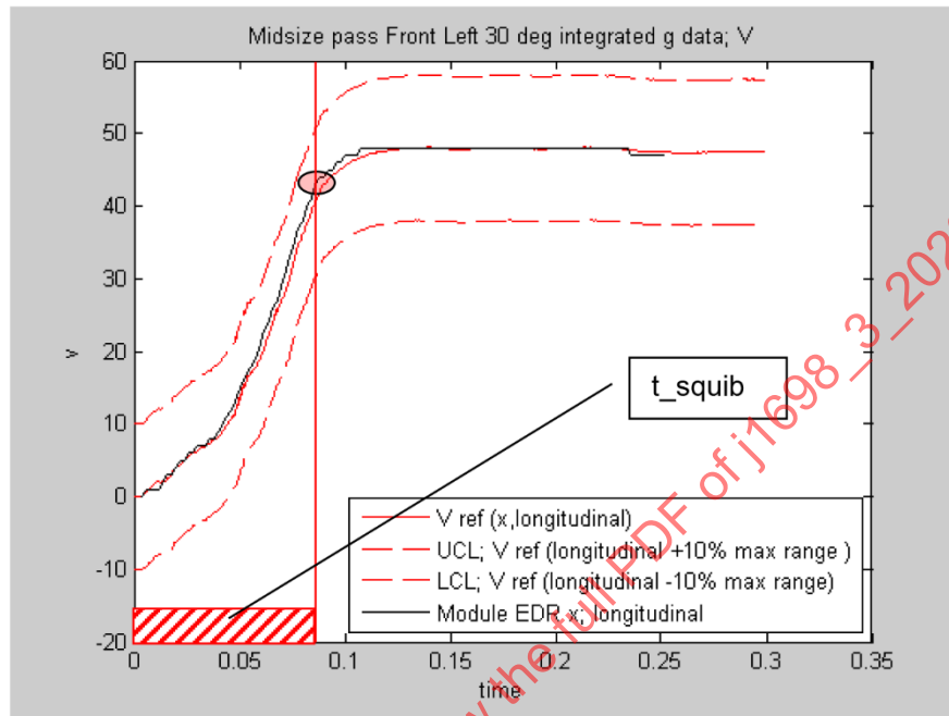
Figure 7 - Example (x) delta velocity signal with t_{squib} alignment
