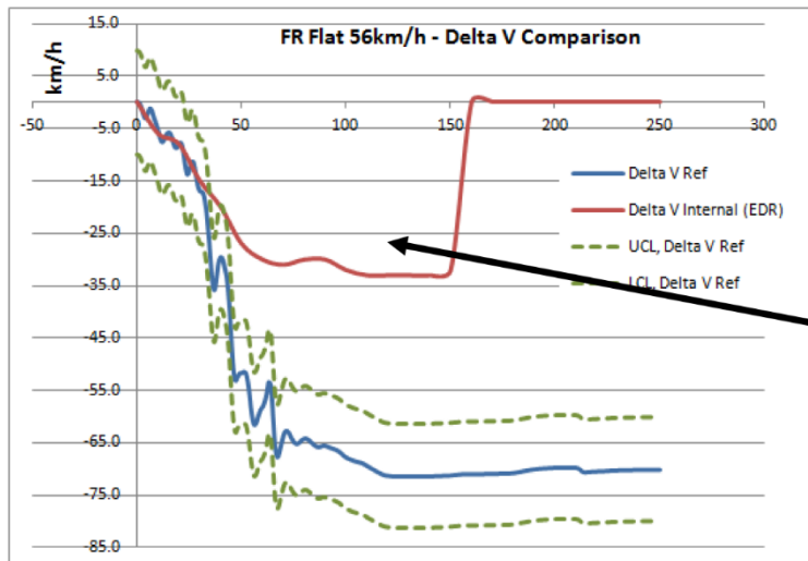
Figure 2 - Example of event with velocity difference based on clipped acceleration signal.
