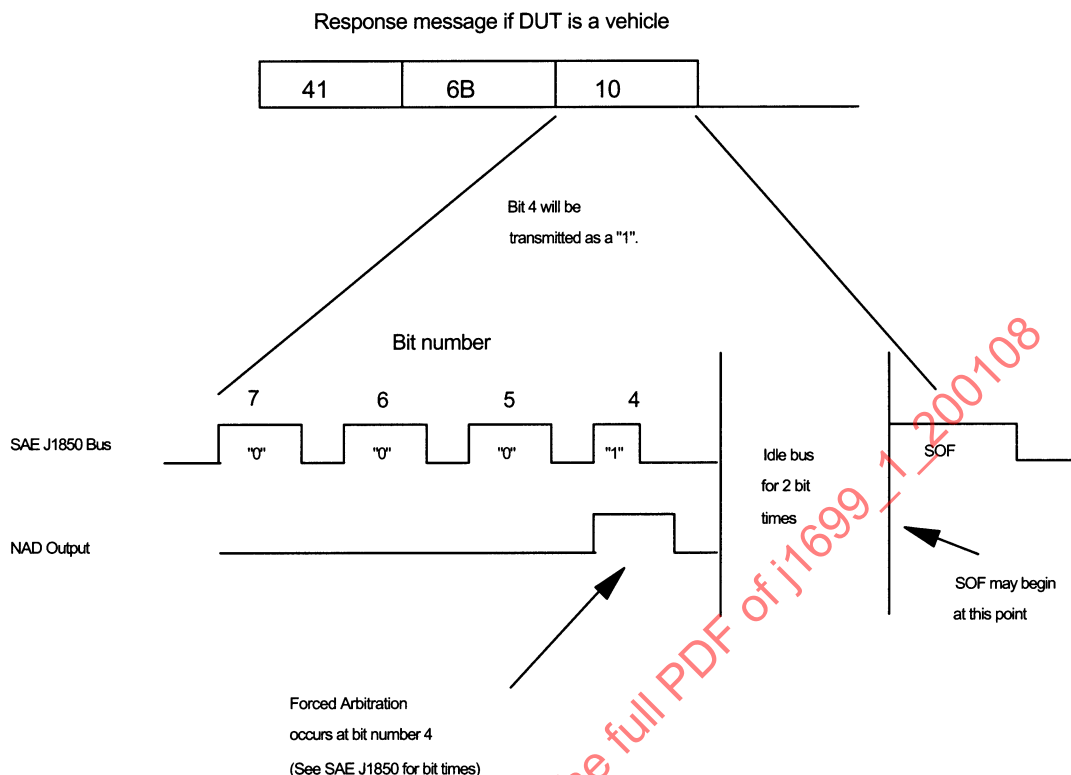
FIGURE 11—FORCED ARBITRATION ON THE THIRD BYTE OF RESPONSE MESSAGE BIT NUMBER 4
