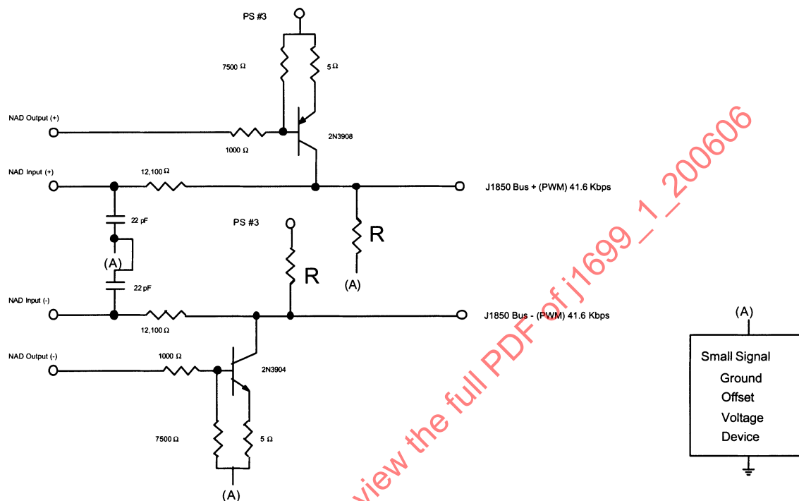
FIGURE 4—PWM BUS RX/TX CIRCUIT
