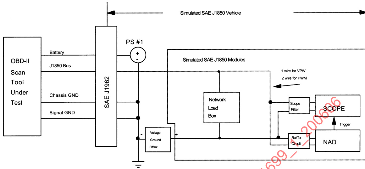
FIGURE 7—OBD-II SCAN TOOL, NEGATIVE GROUND OFFSET FROM SAE J1962 CONNECTOR
