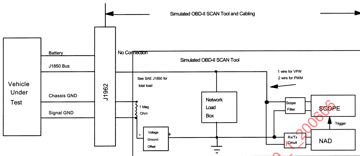
FIGURE 9—VEHICLE, NEGATIVE GROUND FROM THE SAE J1962 CONNECTOR
