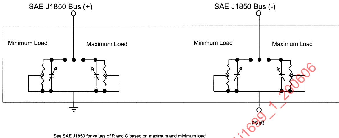
FIGURE 6—SAE J1850 NETWORK LOAD BOX
