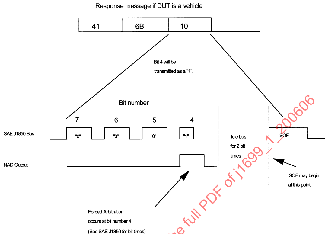
FIGURE 11—FORCED ARBITRATION ON THE THIRD BYTE OF RESPONSE MESSAGE BIT NUMBER 4
