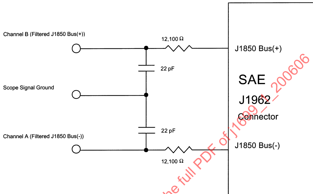
FIGURE 5—PWM SCOPE INPUT FILTER
