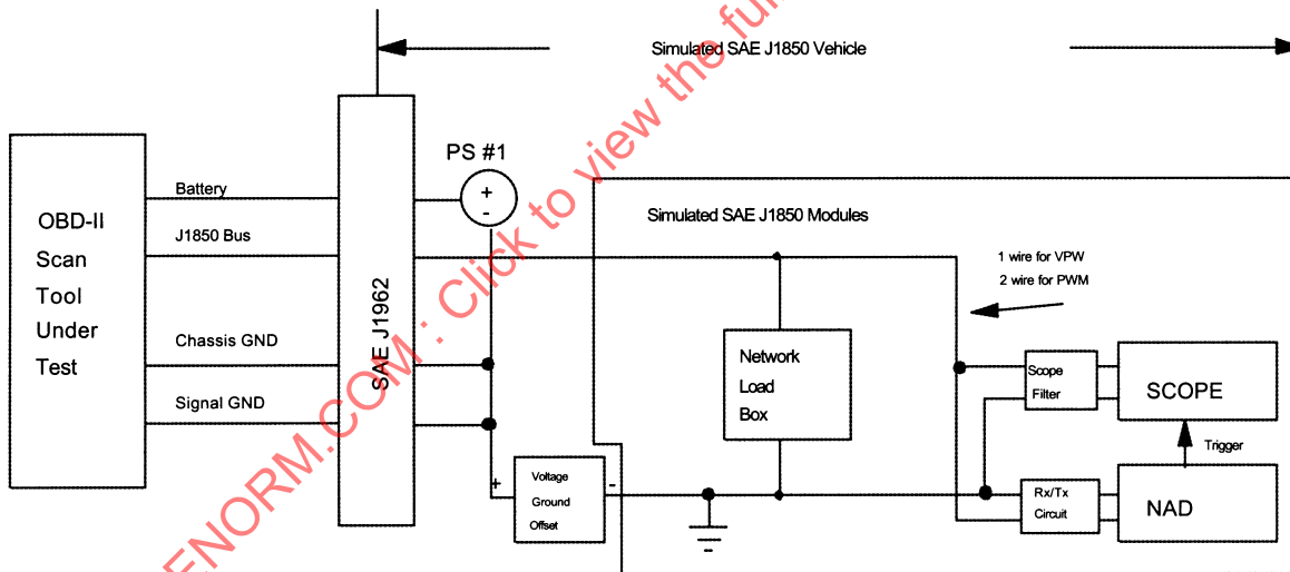
FIGURE 8—OBD-II SCAN TOOL, POSITIVE GROUND OFFSET FROM SAE J1962 CONNECTOR
