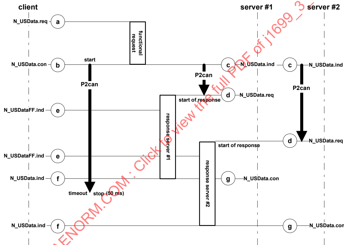
Figure 8 – Functional OBD communication - default response timing
