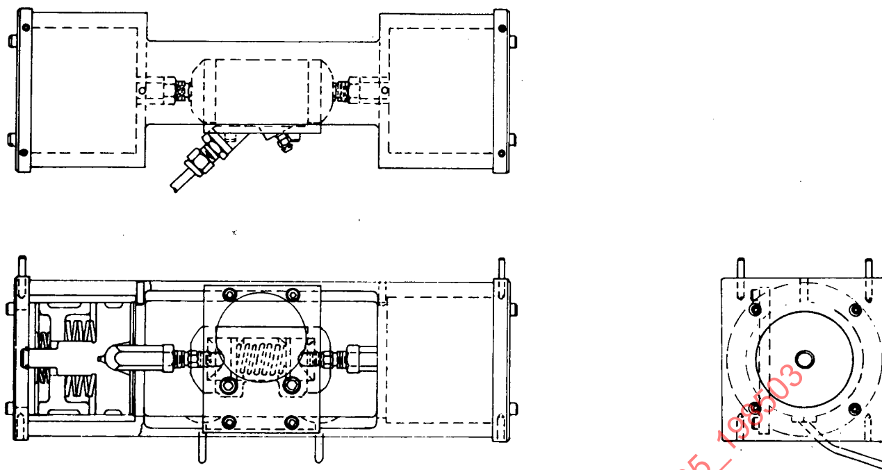
FIG. 2—STROKING FIXTURE APPARATUS
