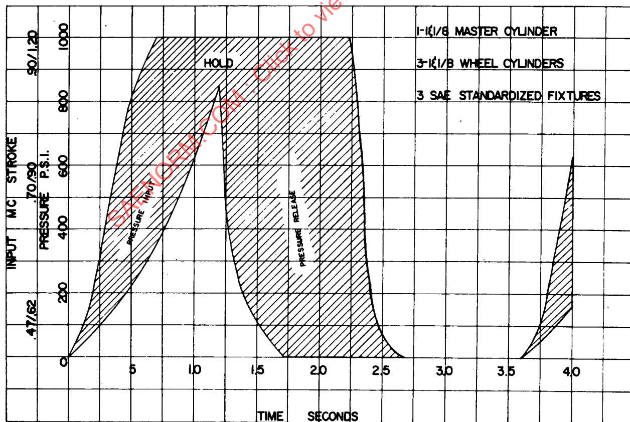
FIG. 3—MASTER CYLINDER STROKE
