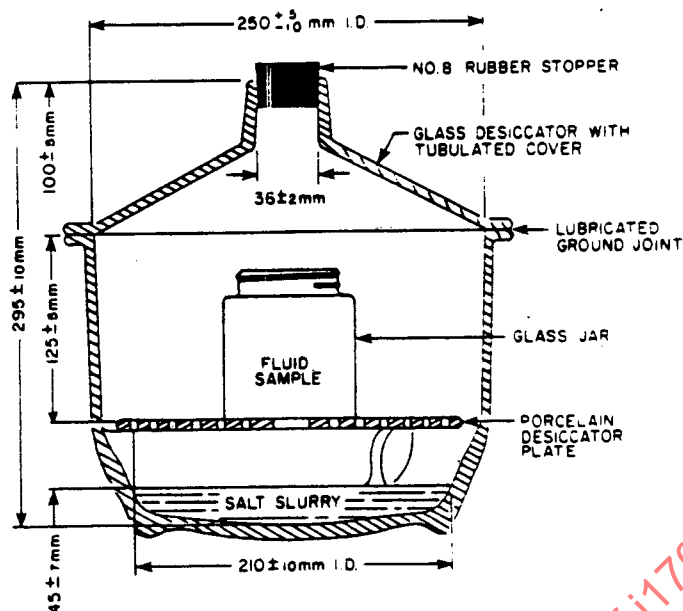
FIGURE 7 - Humidification Apparatus
