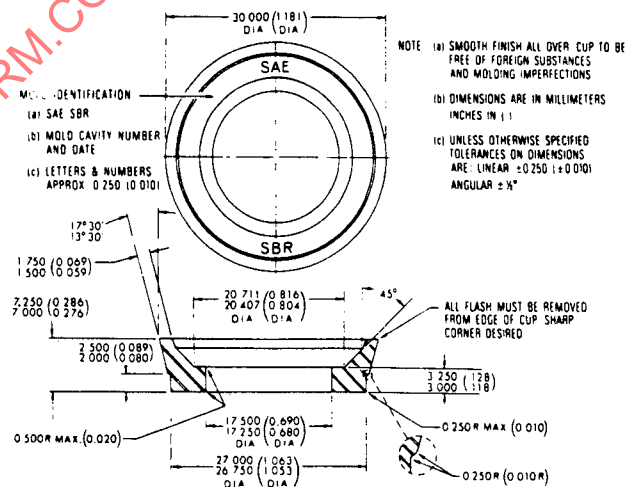
FIGURE 6 - SAE Test Cup - Secondary Master Cylinder
