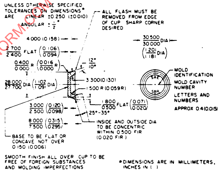
FIGURE 4 - SAE Test Cup Wheel Cylinder
