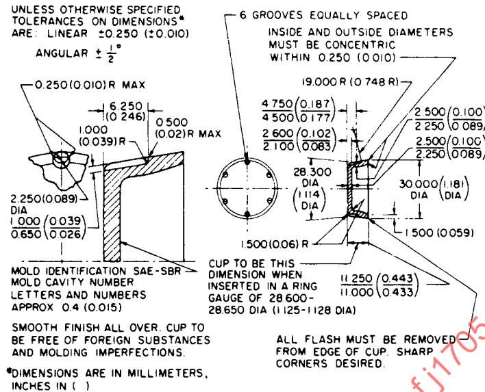
FIGURE 5 - SAE Test Cup - Primary Master Cylinder
