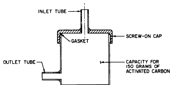
FIG. 1—RECOMMENDED TRAP DESIGN
