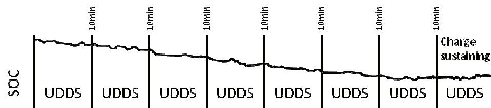
FIGURE 6 - RECOMMENDED UDDS TEST LAYOUT FOR CHARGE-DEPLETING FCT
