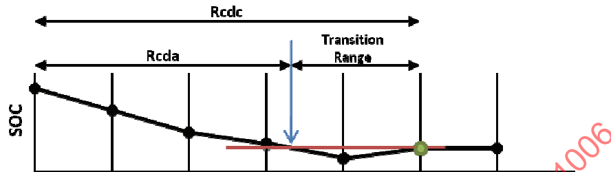
FIGURE 2 - RCDA, RCDC, AND TRANSITIONAL RANGE
