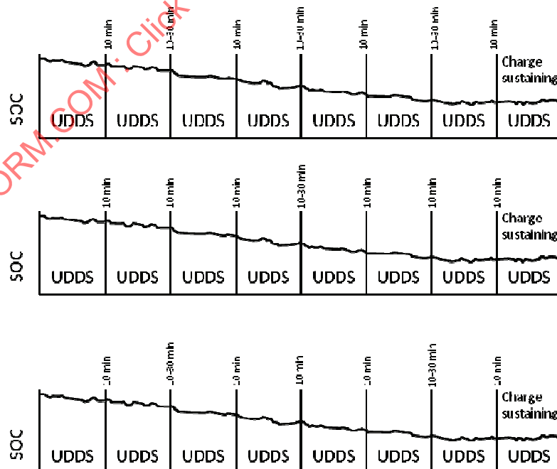
FIGURE 7 - EXAMPLES OF BACKUP TEST OPTIONS USING LONGER SOAK PERIODS DURING SOME INTRA-TEST PAUSES
