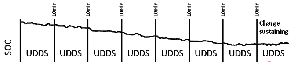
FIGURE 11 - RECOMMENDED TEST LAYOUT FOR COLD UDDS CHARGE-DEPLETING FCT
