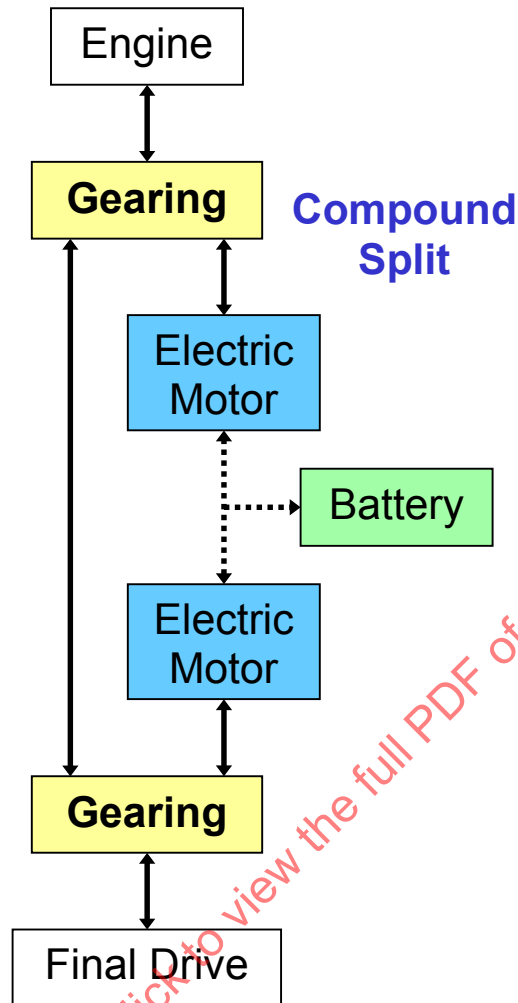
FIGURE 2 - COMPOUND SPLIT
