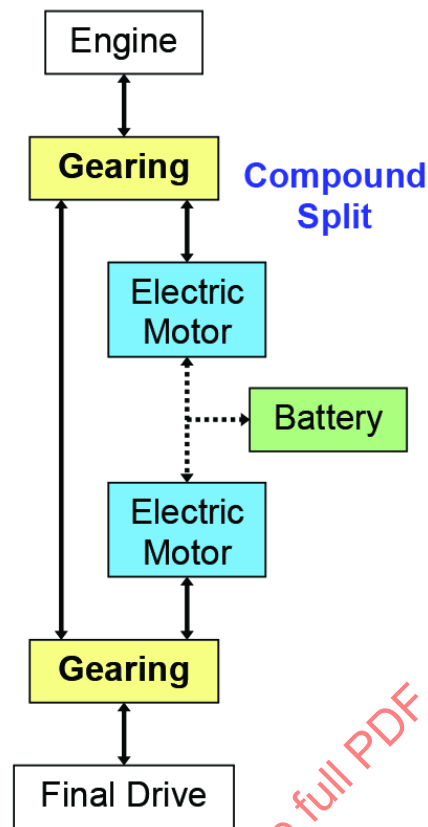
Figure 3 - Compound split
