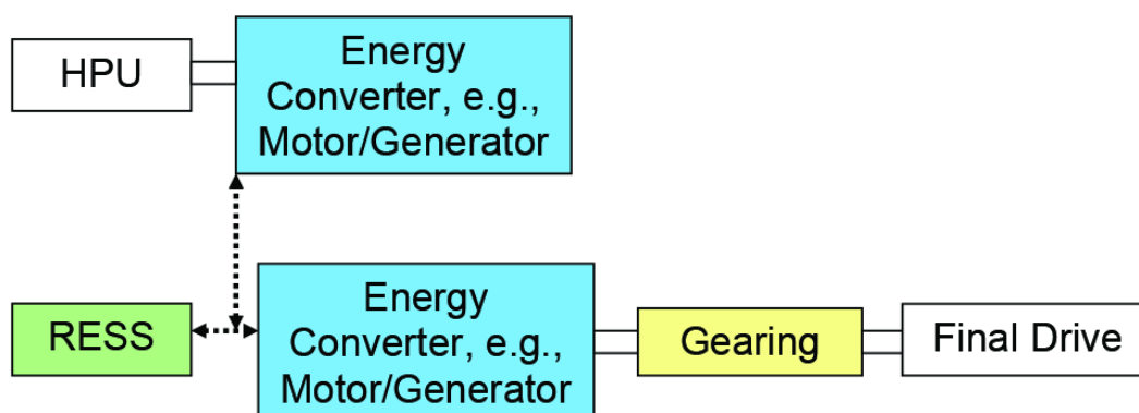
Figure 4 - Series hybrid
