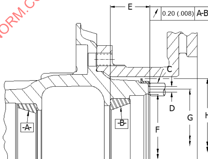
Figure 5 - R, N, and P disc brake application U rotor
