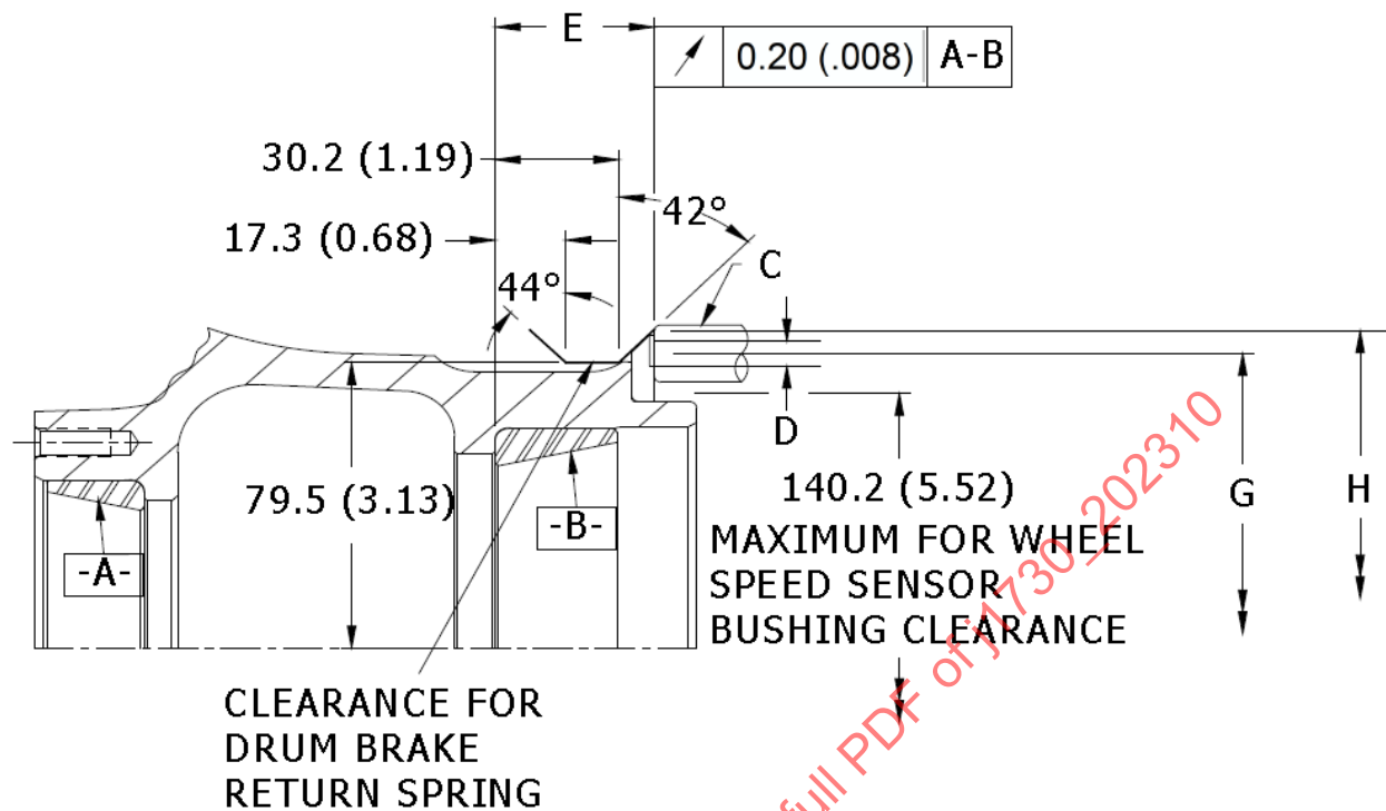
Figure 2 - FF drum brake application
