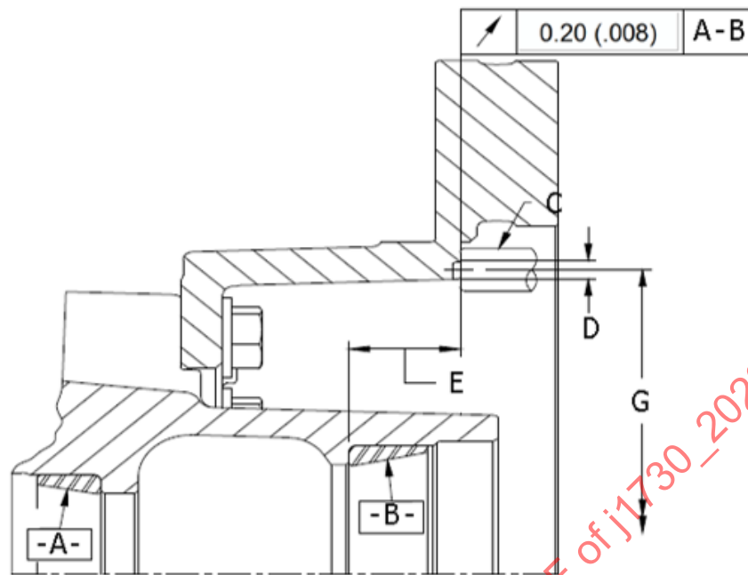
Figure 8 - FC, FF, and FL disc brake application hat rotor
