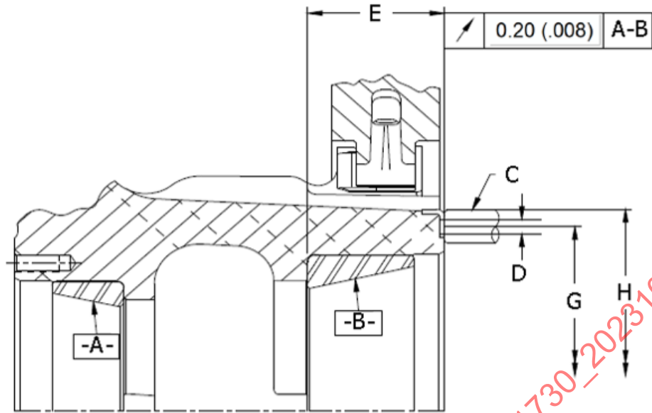
Figure 10 - FF and FL disc brake application flat rotor
