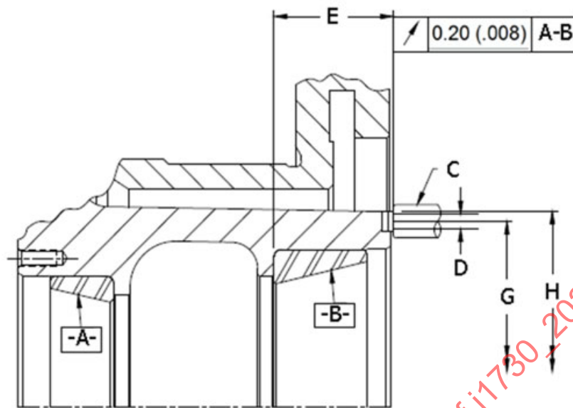
Figure 6 - FF, FH, and FL disc brake application U rotor
