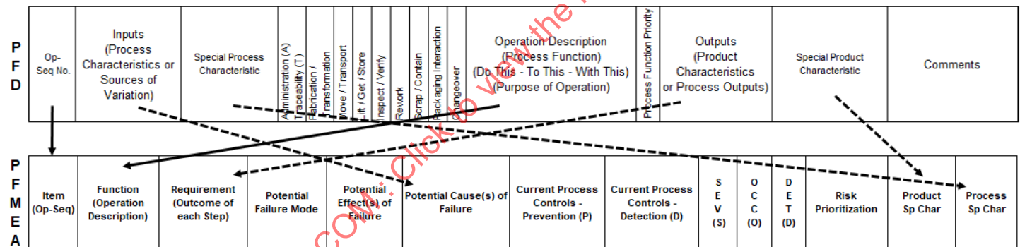
Figure 35 - PFD and PFMEA connection
