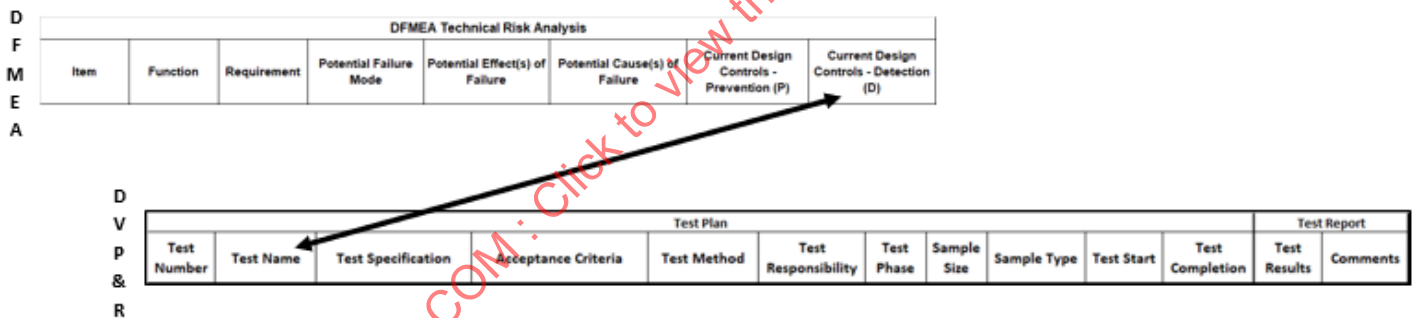
Figure 29 - DFMEA and DVP&R connection
