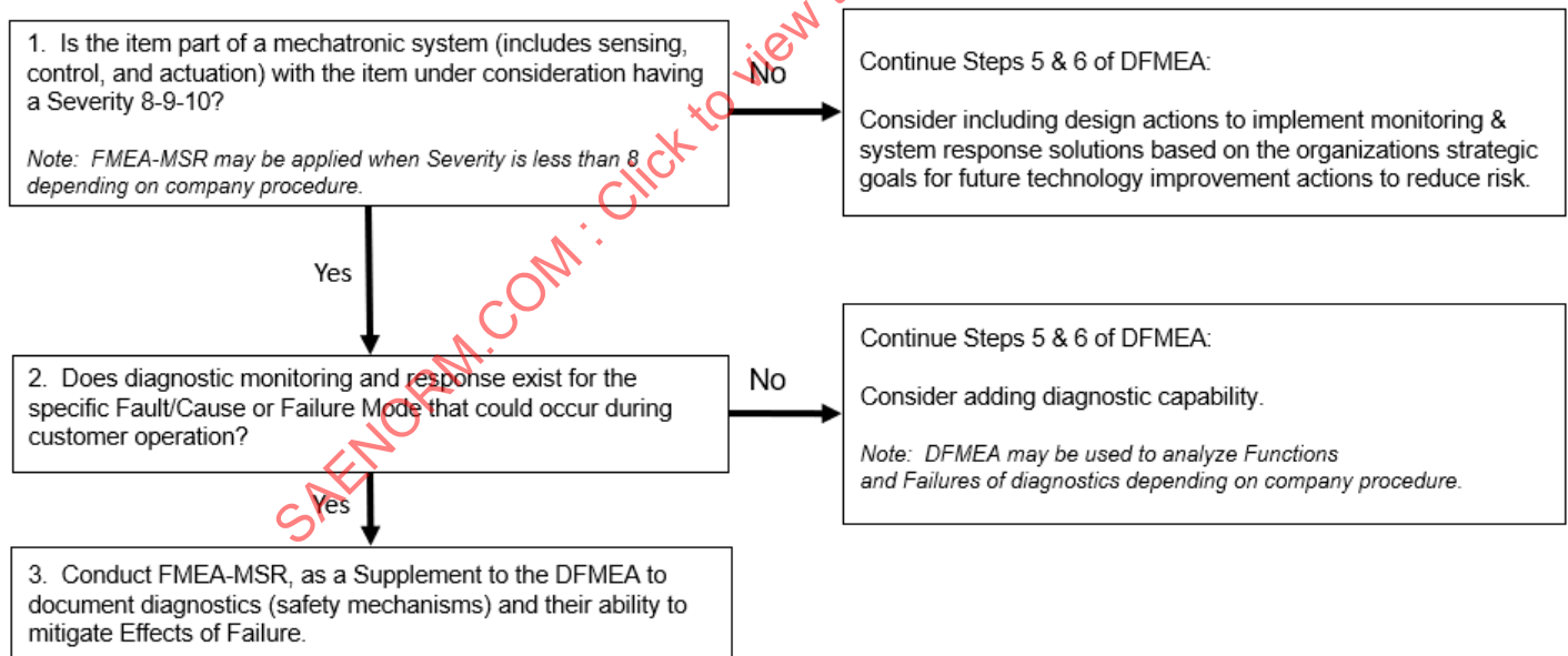
Figure 18 - FMEA-MSR decision-making process
