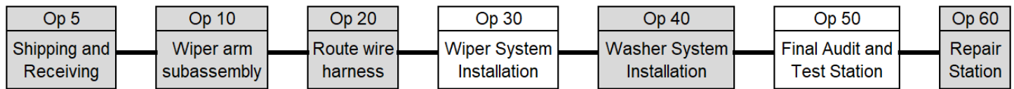
Figure 32 - Preliminary risk assessment defines windshield wiper system macro operations requiring PFMEA
