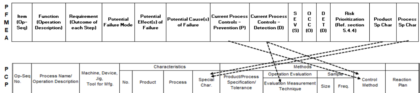
Figure 51 - PFMEA and PCP connection
