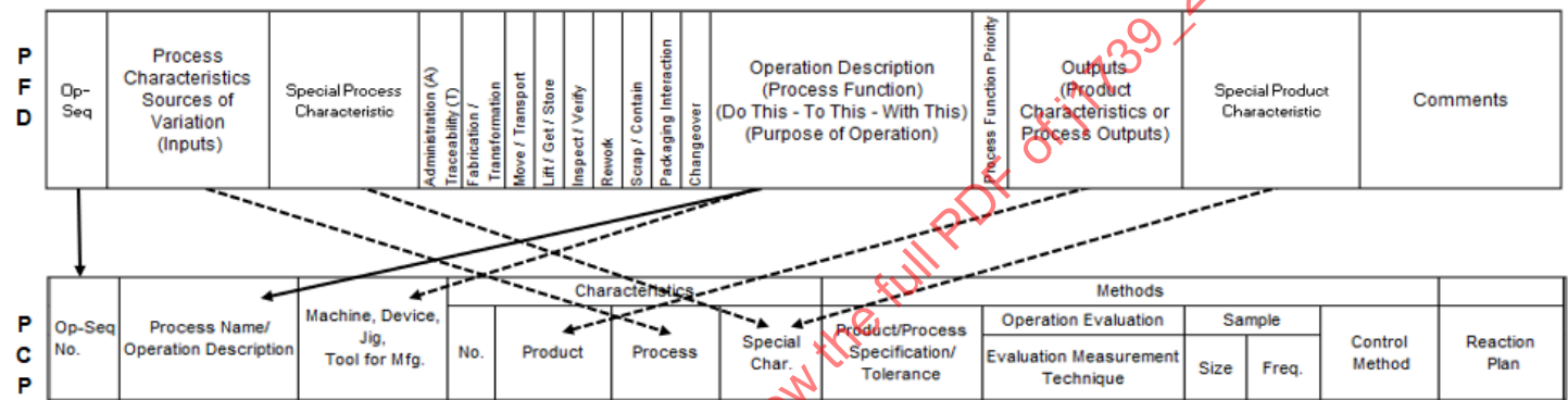
Figure 50 - PFD and PCP connection
