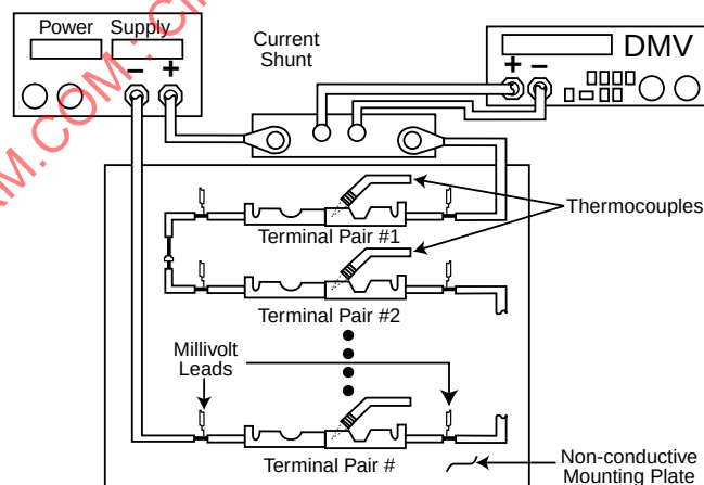
FIGURE 3 - SET-UP FOR MAXIMUM TEST CURRENT
