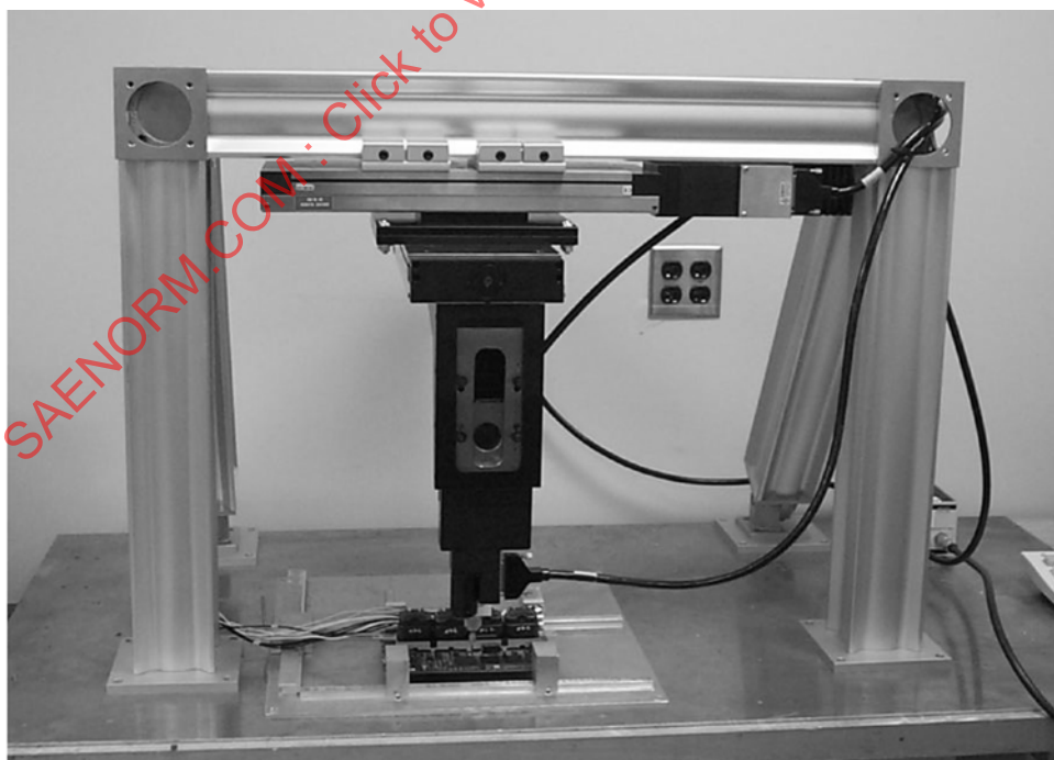
FIGURE 4—X, Y AND Z POSITIONER
