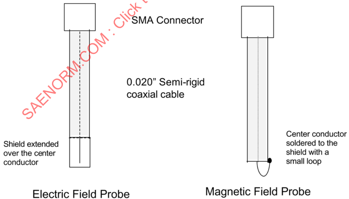
FIGURE 2—DRAWING OF TYPICAL SCAN PROBES
