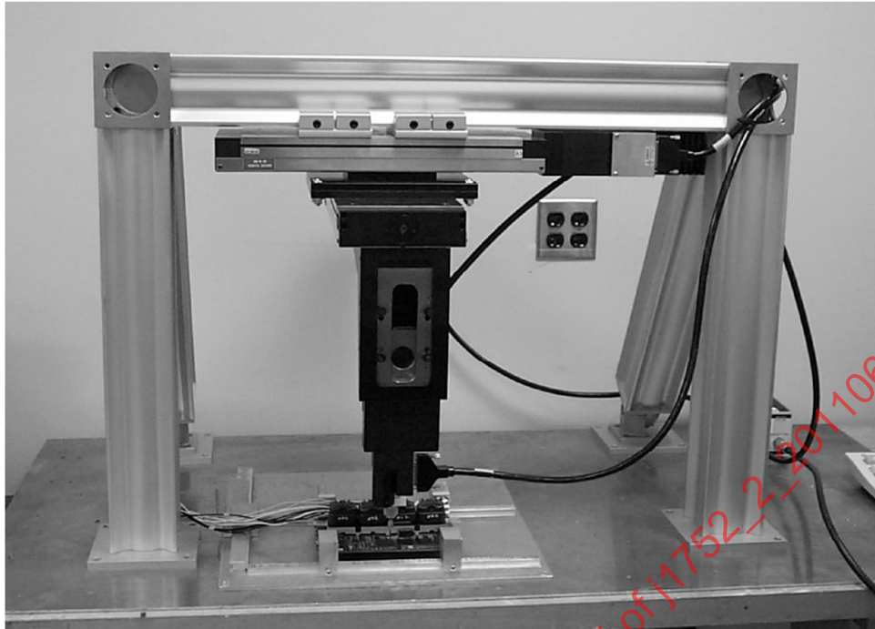
FIGURE 3 - X, Y AND Z POSITIONER
