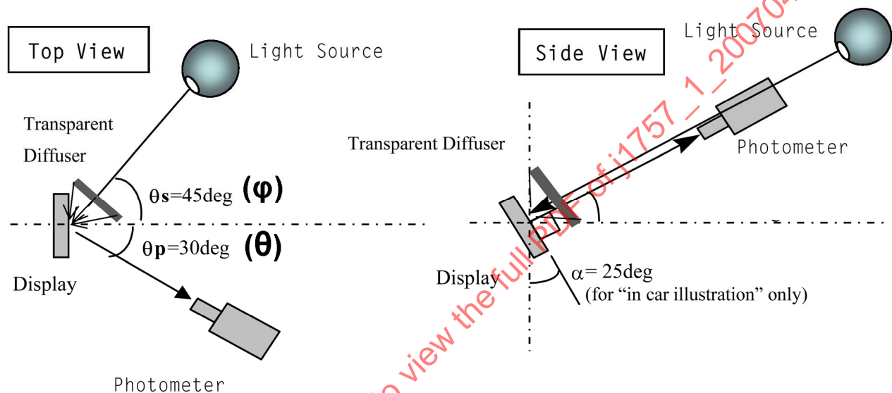
FIGURE 5 - SET-UP "2B" FOR HIGH AMBIENT CONTRAST MEASUREMENT
