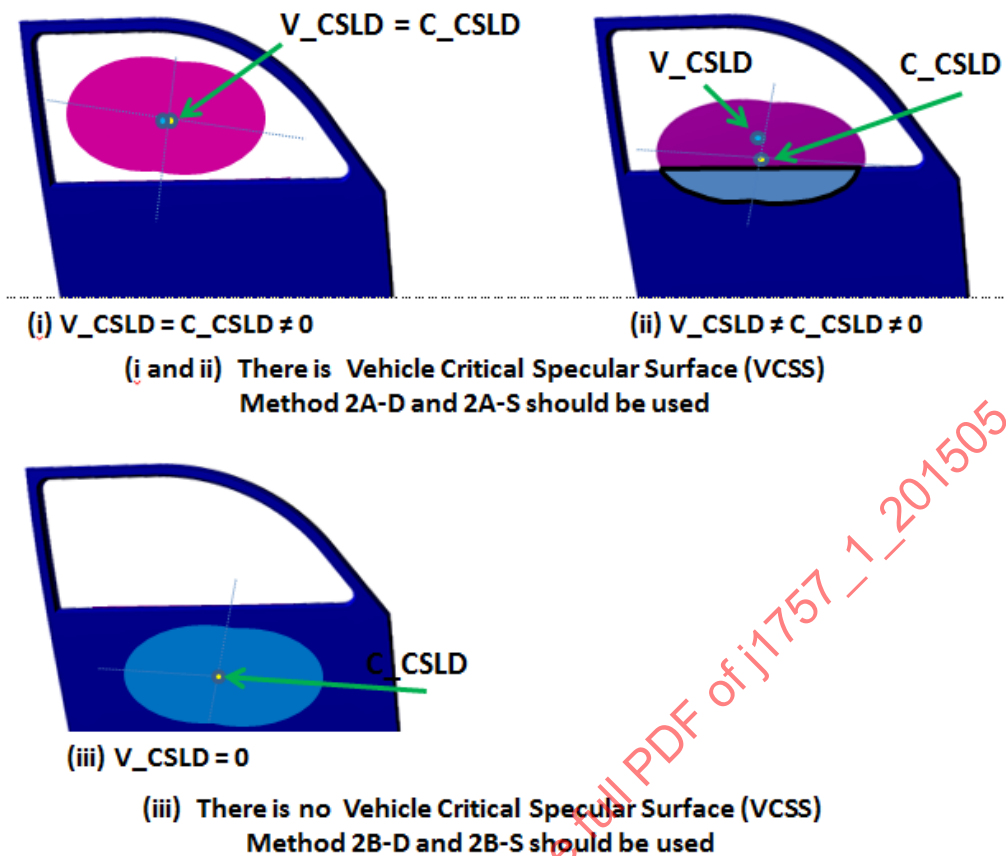
Figure 1B - Critical light illumination examples
