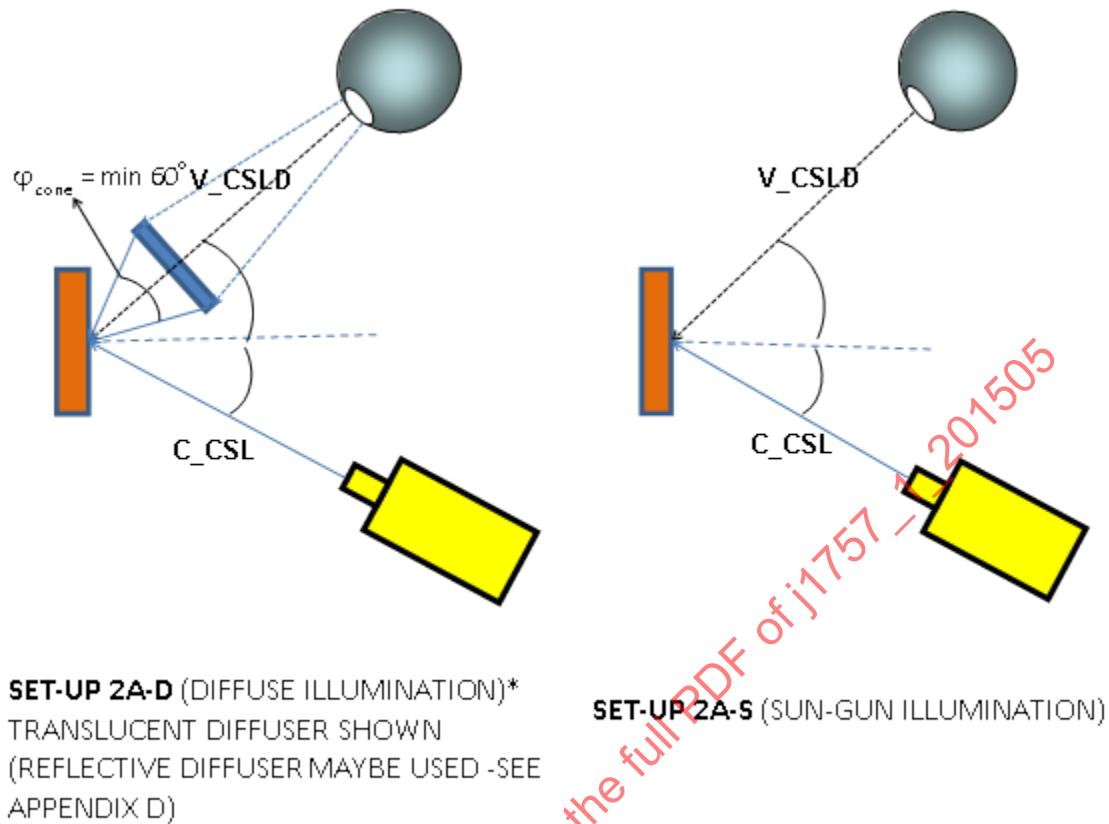
Figure 4 - Set-up for Method 2A
