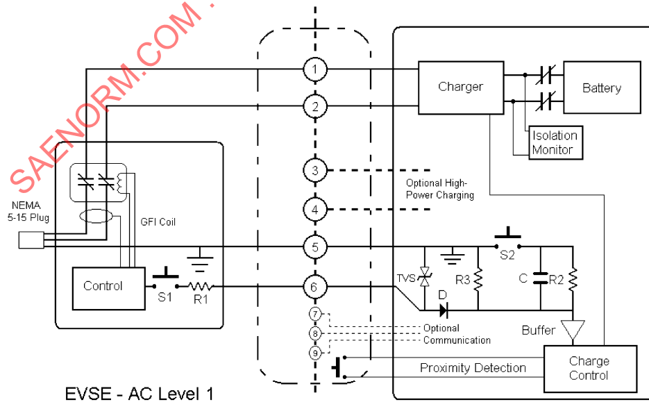
FIGURE 4—AC LEVEL 1 SYSTEM CONFIGURATION
