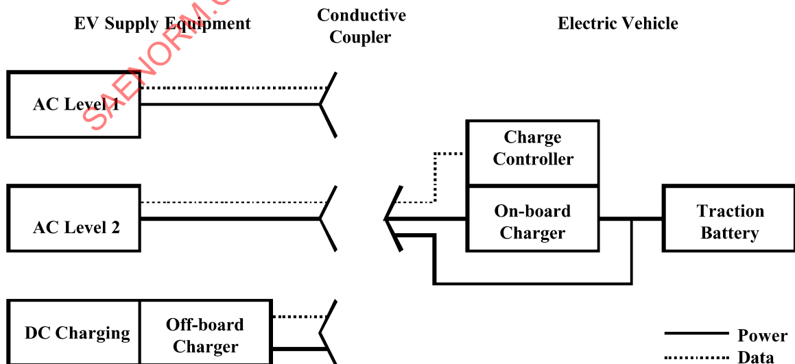
FIGURE 1—CONDUCTIVE EV CHARGING SYSTEM ARCHITECTURE
