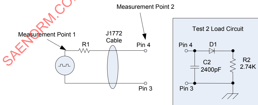
FIGURE C.4.2: PILOT PIN LOADING DIAGRAM
