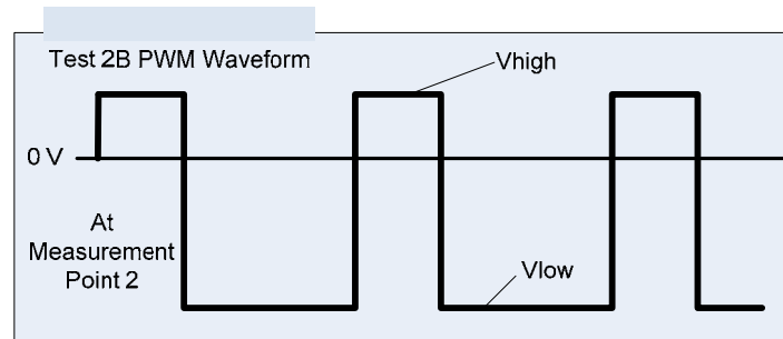
FIGURE C.4.2.2: ANTICIPATED WAVEFORM AT MEASUREMENT POINT 2
