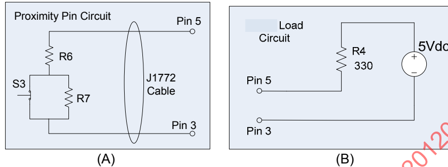
FIGURE C.7.1: PROXIMITY PIN CIRCUIT (A) AND TEST LOAD CIRCUIT (B)
