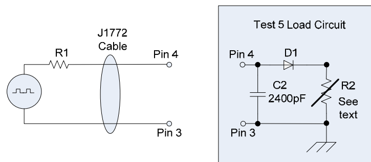
FIGURE C.5.1: PILOT PIN LOADING DIAGRAM
