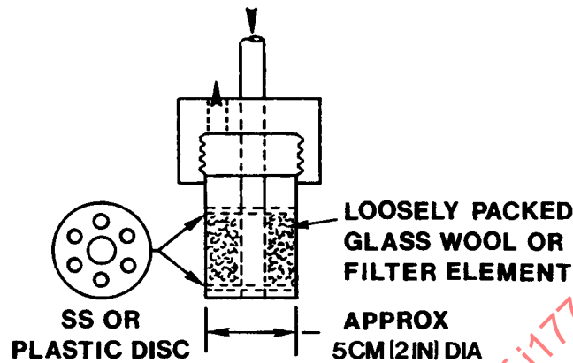
FIGURE 3—PREFILTER, F3, OR SOOT KNOCKOUT TRAP (EXAMPLE)
