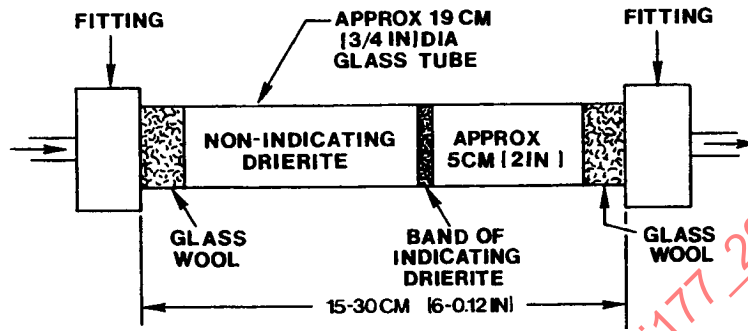
FIGURE 2—DRYING TUBE (EXAMPLE)
