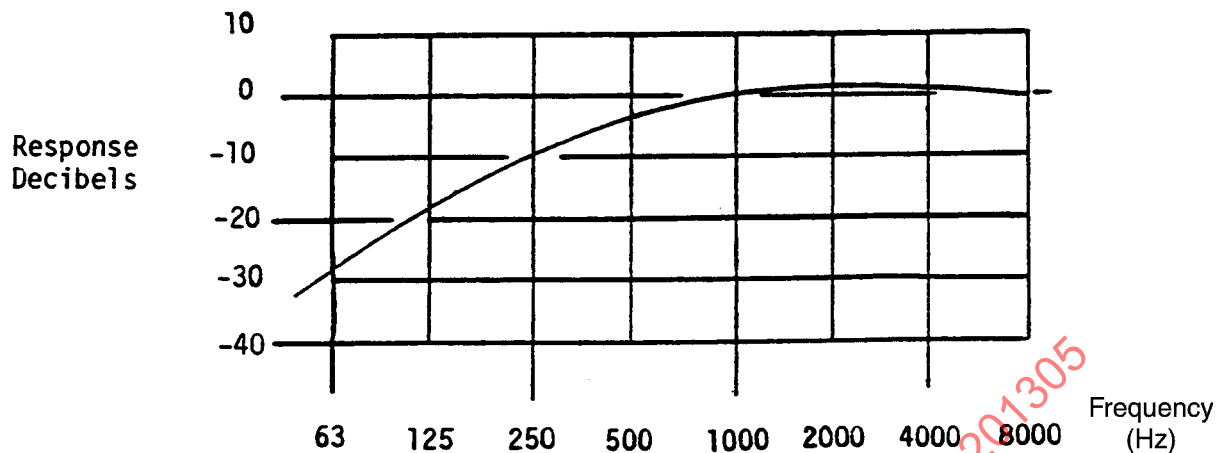
FIGURE 2—CHARACTERISTICS OF A STANDARD A FILTER
