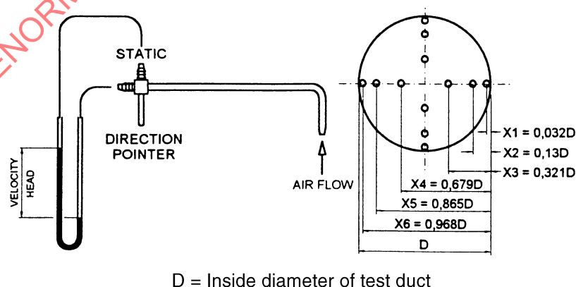
Figure 3 - Pitot tube positions for a six-point pass in circular ducts
