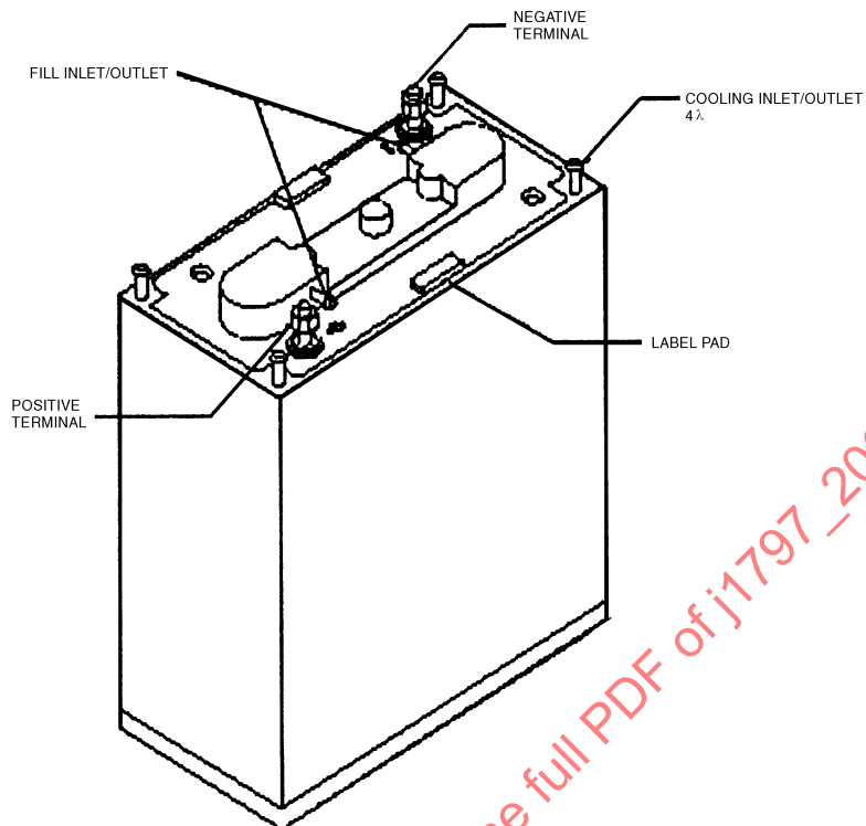
FIGURE 3A—ISOMETRIC VIEW
