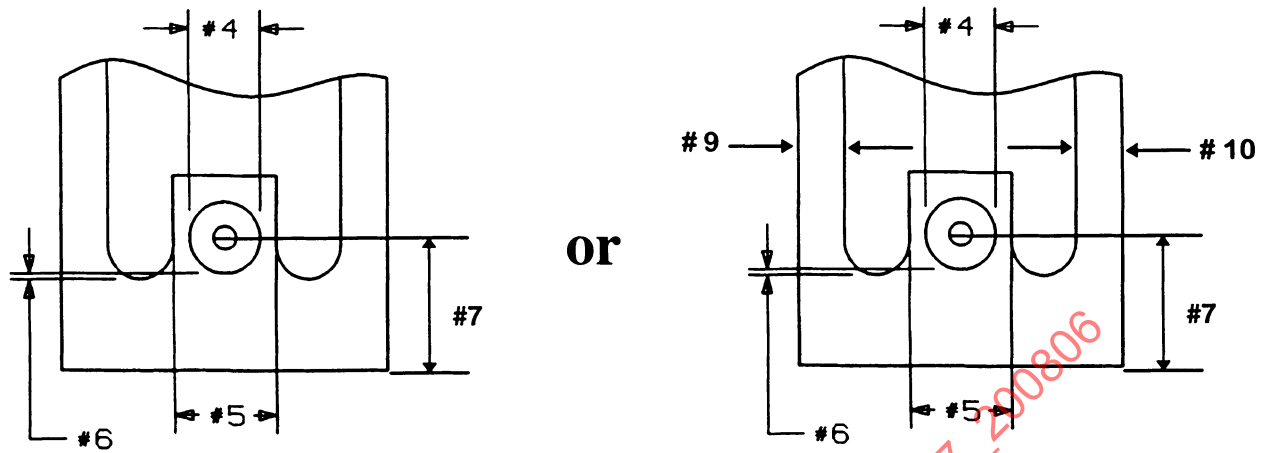
FIGURE 1F—TOP VIEW
