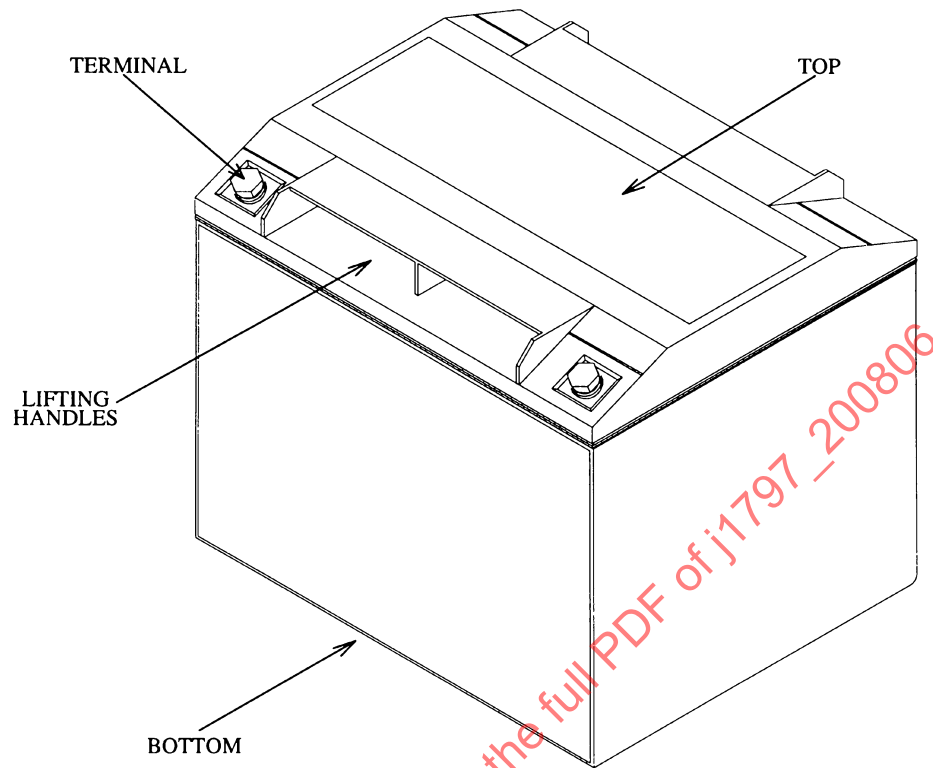
FIGURE 4A—ISOMETRIC VIEW
