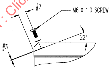
FIGURE 4E—TERMINAL END VIEW
