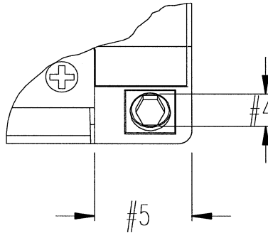
FIGURE 4F—TERMINAL TOP VIEW
