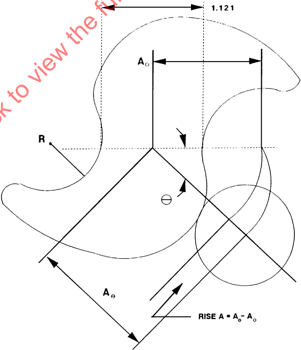
FIGURE C9—CAM PROFILE
