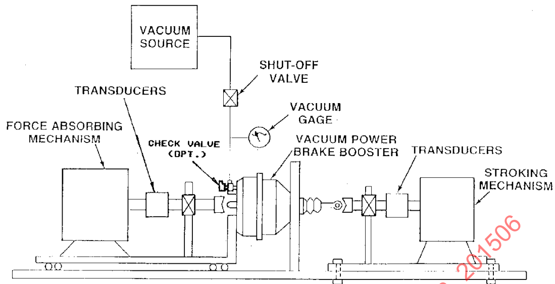
Figure 2 - Schematic of recommended setup
