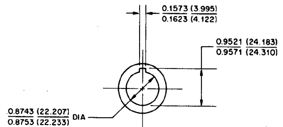
FIG. 4-PULLEY HUB DIMENSIONS
