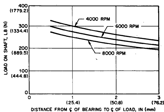
FIG. 9—TYPICAL CHART FOR SHOWING LIMITATIONS FOR SHAFT LOADING
