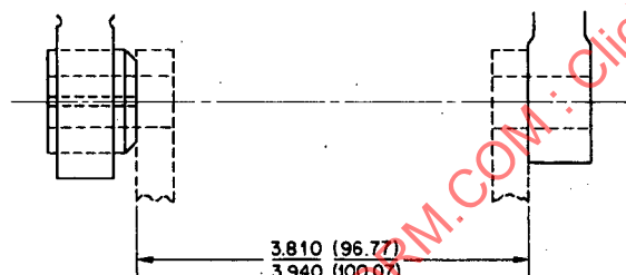
FIG. 7—TYPICAL INSTALLATION OF SPLIT BUSHING IN HINGE MOUNTING LUG
