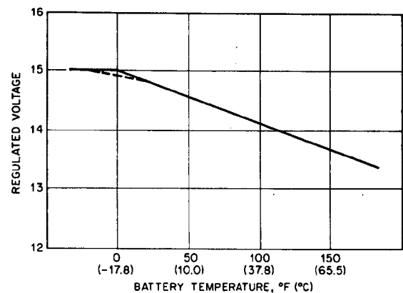
FIG. 5-NOMINAL REGULATOR COMPENSATION CURVE
