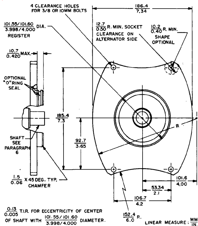
φ FIG. 12—ALTERNATOR FLANGE MOUNT. FOUR BOLT—AIR COOLED
