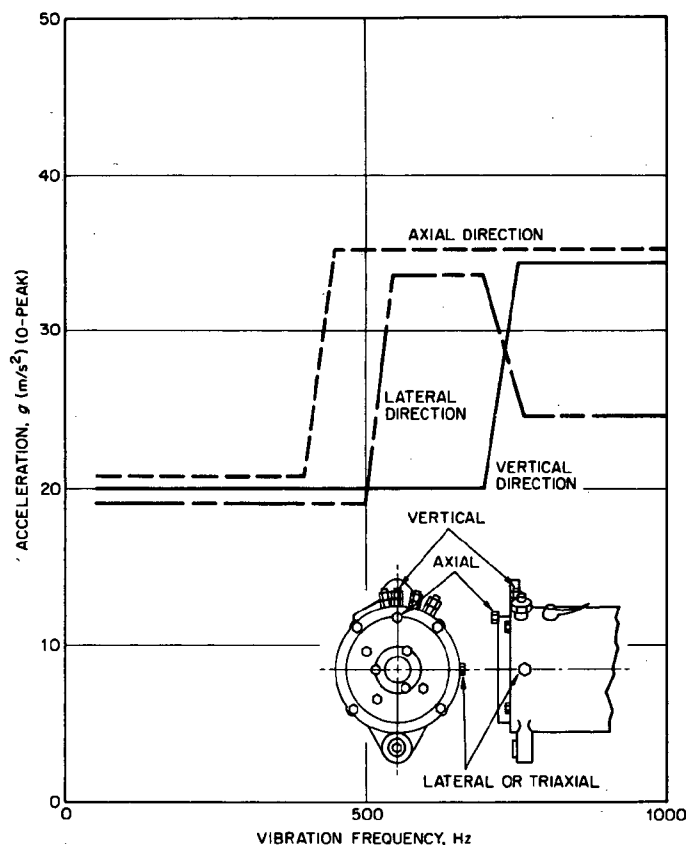
FIG. 6—VIBRATION TOLERANCE CURVE
