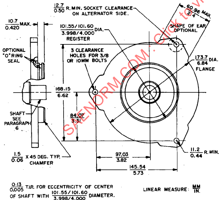
φ FIG. 11—ALTERNATOR FLANGE MOUNT. THREE BOLT—AIR COOLED
