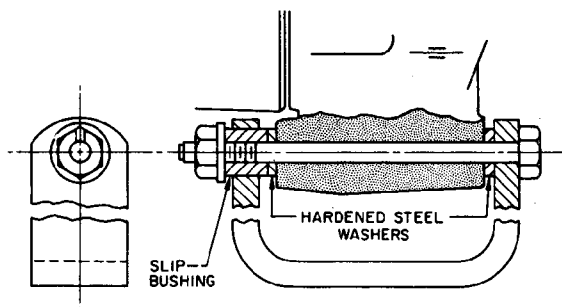
FIG. 8—TYPICAL INSTALLATION OF SPLIT BUSHING IN BRACKET FOR SPOOL MOUNTING
