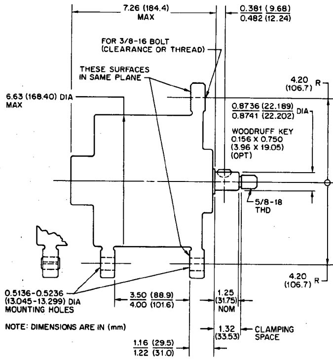
DOUBLE-LUG MOUNTING
