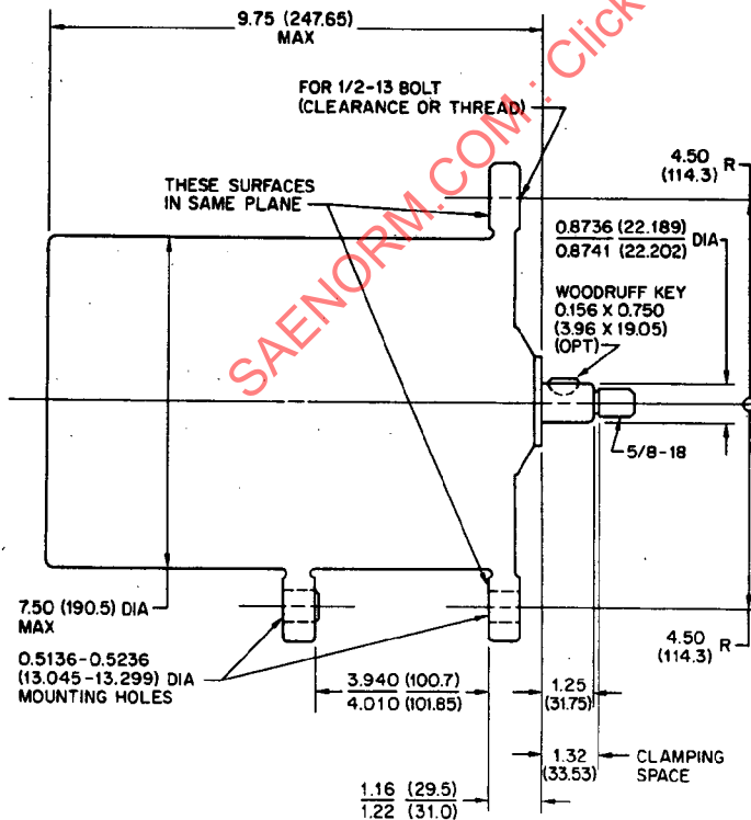
FIG. 3-ENVELOPE FOR MACHINE WITH ENCLOSED REGULATOR AND DIODES
