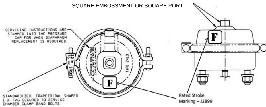
Figure 2 - 76.2 mm (3.00 inches) long-stroke actuator identification
