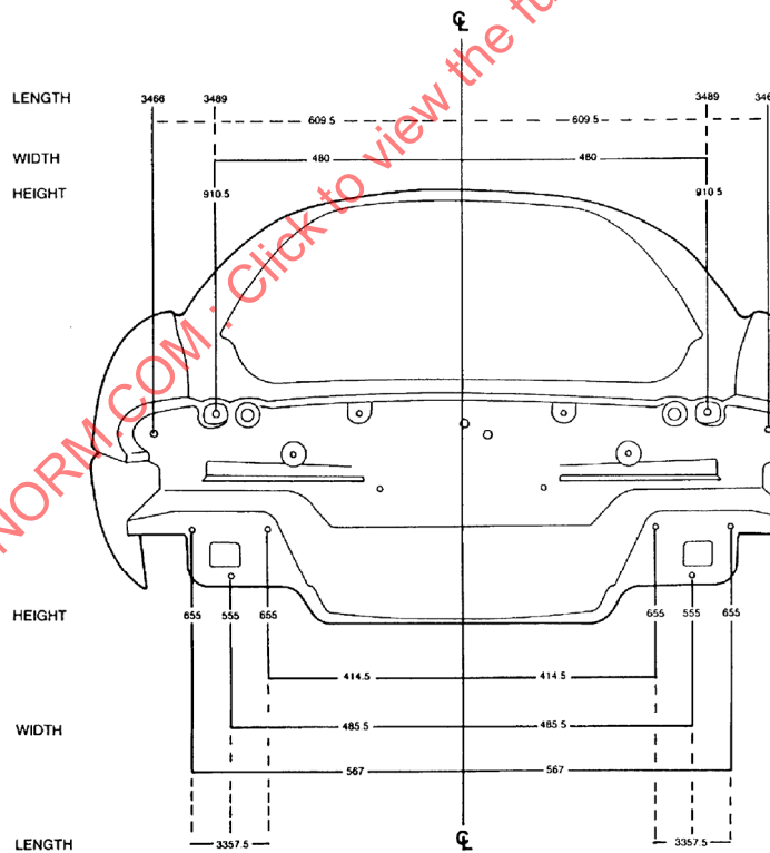
FIGURE 5 - REAR VIEW
