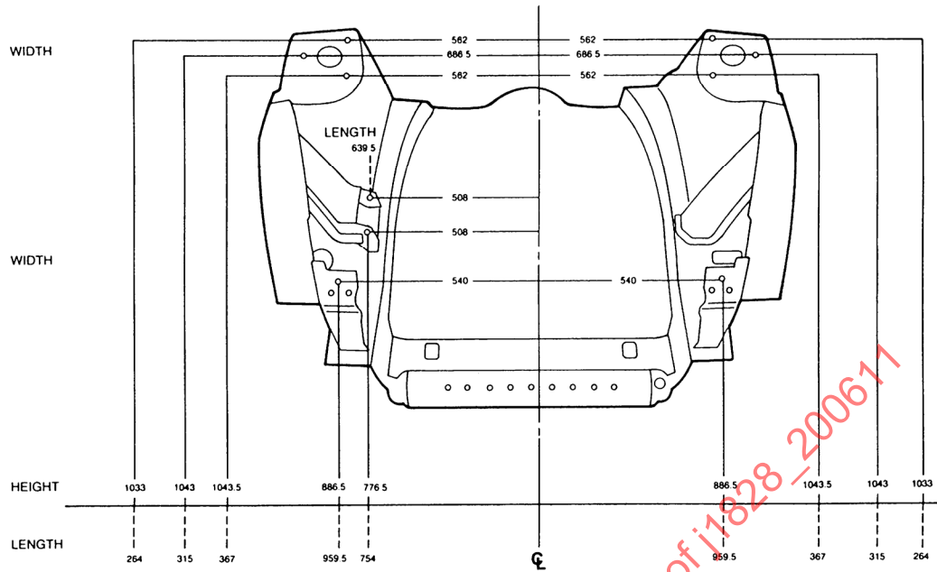
FIGURE 6 - ENGINE COMPARTMENT VIEW
