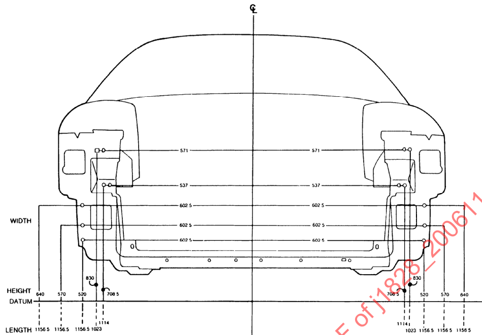
FIGURE 4 - FRONT VIEW
