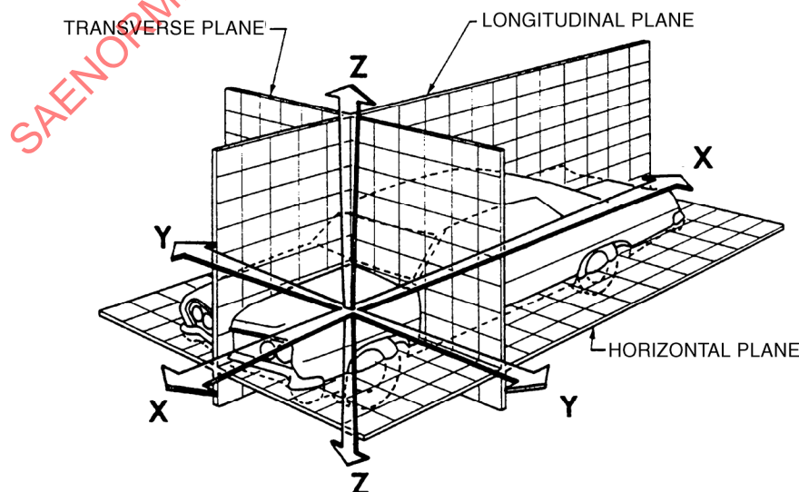
FIGURE 1 - DATUM PLANES
