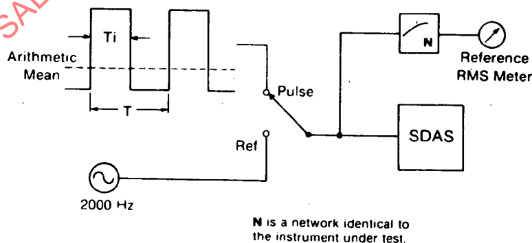
FIG.8 - RECTANGULAR PULSE TEST
