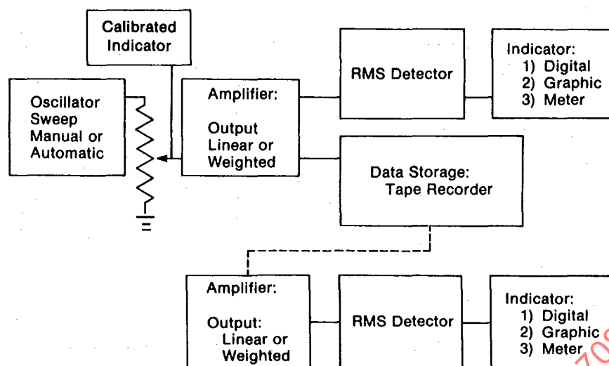
FIG. 3—FREQUENCY RESPONSE QUALIFICATION
