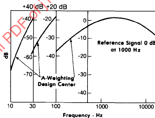
FIG. 4—STEP INCREASES IN SYSTEM INTERNAL SIGNAL TO KEEP A-WEIGHTING RESPONSE VERIFICATION ABOVE SYSTEM ELECTRONIC NOISE FLOOR
