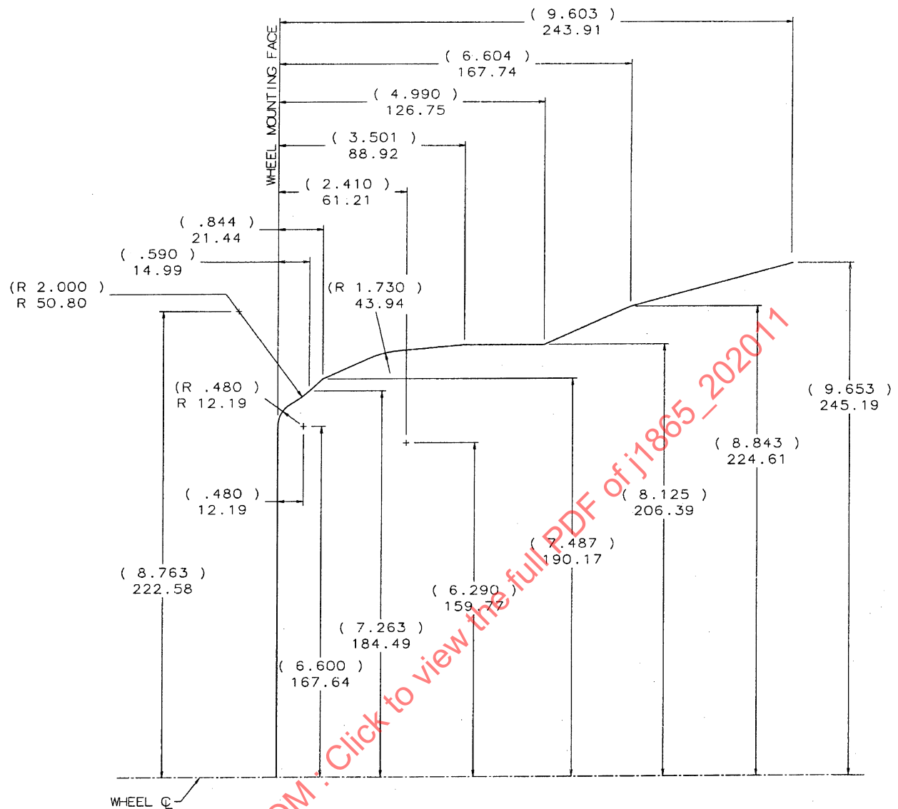
Figure 1- Clearance line:19.5 x 6.75 wheels, mounting system ii
