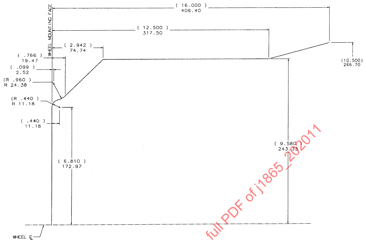
Figure 4 - Clearance line: 22.5 x 7.50, 8.25, and 9.00 wheels, mounting systems iii and xiv 24.5 x 8.25 wheels, mounting systems iii and xiv
