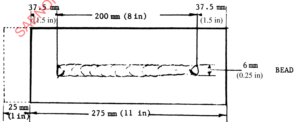
FIGURE 7—VERTICAL EXPANSION SAMPLE/SUBSTRATE GEOMETRY
