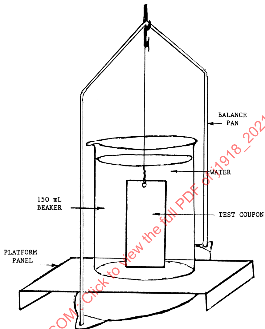
FIGURE 3—ANALYTICAL SCALE SET-UP
