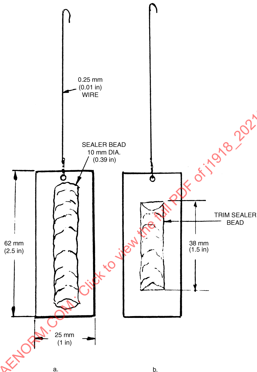
FIGURE 4—GRAVIMETRIC EXPANSION SAMPLE AND COUPON GEOMETRY
