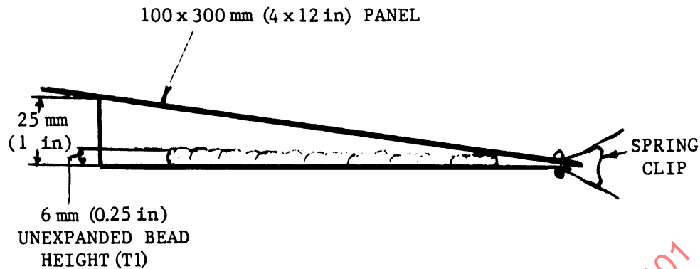
FIGURE 8—VERTICAL EXPANSION PRE-BAKE SAMPLE PREPARATION
