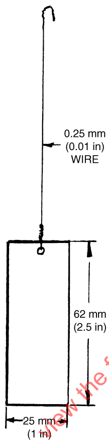
FIGURE 2—COUPON ASSEMBLY
