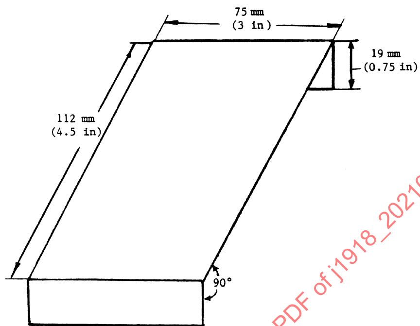
FIGURE 1—PLATFORM PANEL
