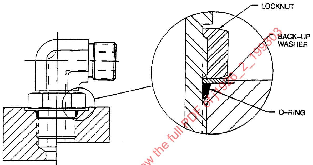
FIGURE B5—FINAL ASSEMBLY OF ADJUSTABLE STUD END
