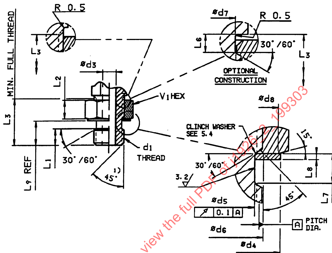
FIGURE 1A—ADJUSTABLE SAE J1926/2 HEAVY-DUTY (S SERIES) STUD END DETAIL
