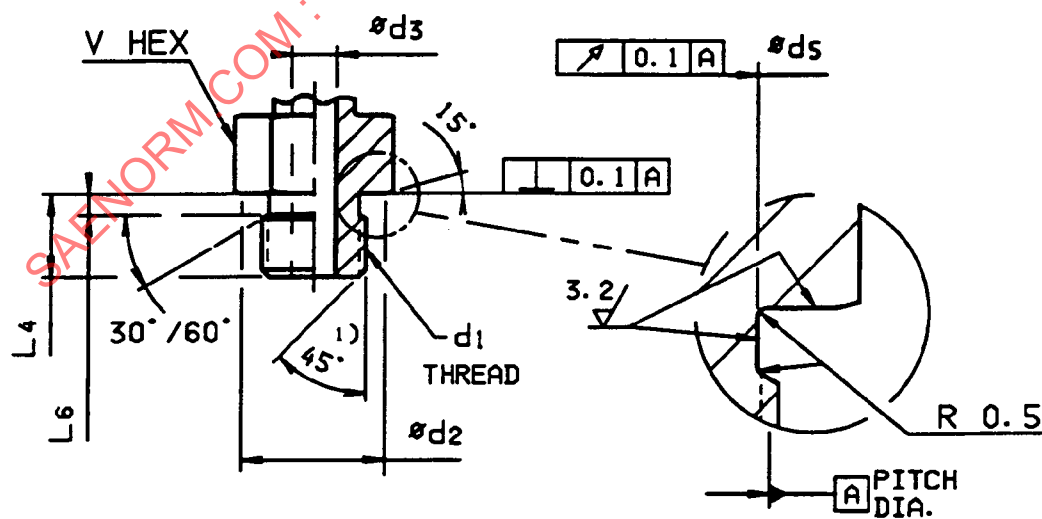
FIGURE 1B—NONADJUSTABLE SAE J1926/2 HEAVY-DUTY (S SERIES) STUD END DETAIL
