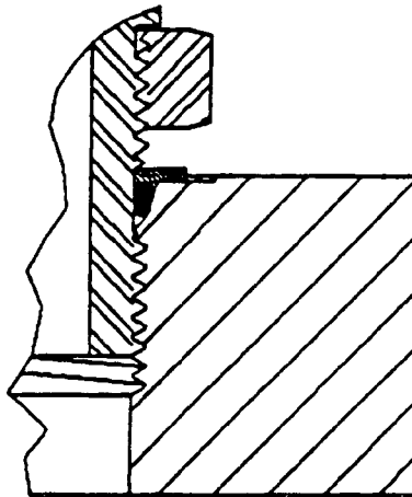
FIGURE B2—FITTING INSTALLED HAND TIGHT
