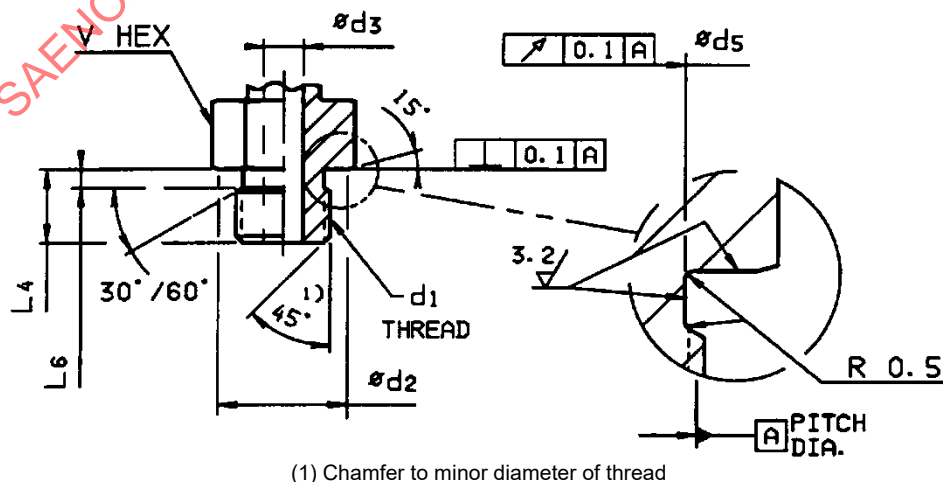
Figure 1B - Nonadjustable SAE J1926-2 heavy-duty (S series) stud end detail
